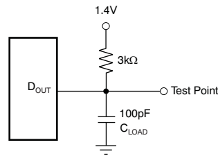
Load Circuit for t_{rD} , t_r , and t_f
