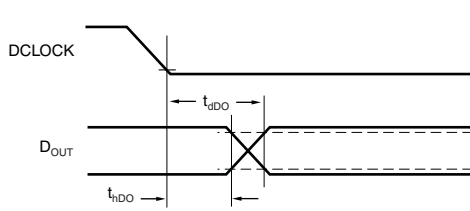
Voltage Waveforms for D_{OUT} Delay Times, t_{dD}
