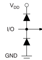
Equivalent Digital Input/Output Circuit
