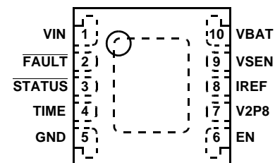
ISL9203 (3x3 DFN) TOP VIEW
