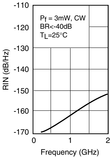
Fig. 7 RIN Characteristics
