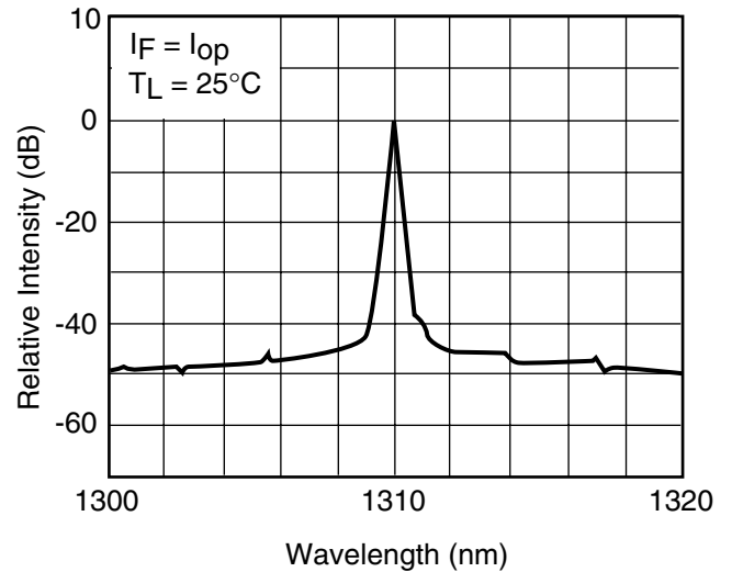
Fig. 4 Lasing Spectrum
