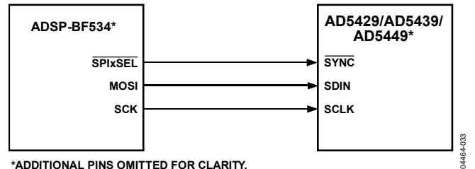
*ADDITIONAL PINS OMITTED FOR CLARITY. Figure 49. ADSP-BF534-to-AD5429/AD5439/AD5449 Interface
