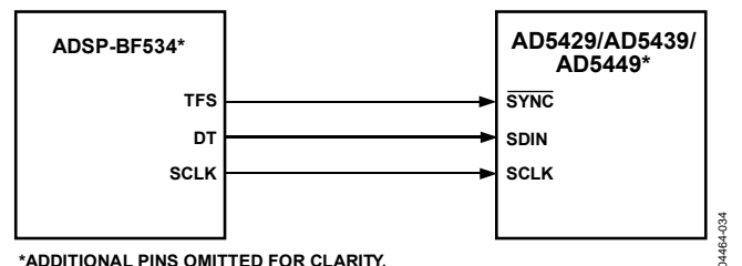
*ADDITIONAL PINS OMITTED FOR CLARITY. Figure 50. ADSP-BF534 SPORT-to-AD5429/AD5439/AD5449 Interface
