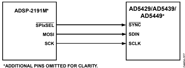
*ADDITIONAL PINS OMITTED FOR CLARITY. Figure 47. ADSP-2191M SPI-to-AD5429/AD5439/AD5449 Interface
