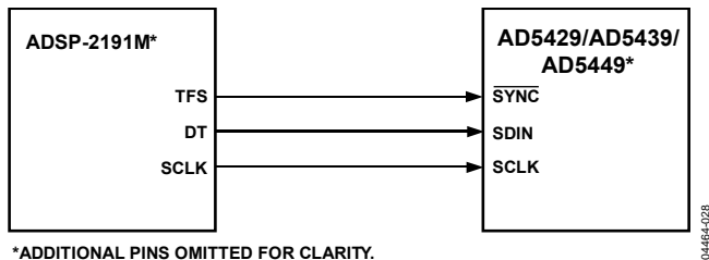
*ADDITIONAL PINS OMITTED FOR CLARITY. Figure 48. ADSP-2191M SPORT-to-AD5429/AD5439/AD5449 Interface
