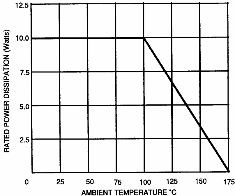
Temperature Rating Curve
