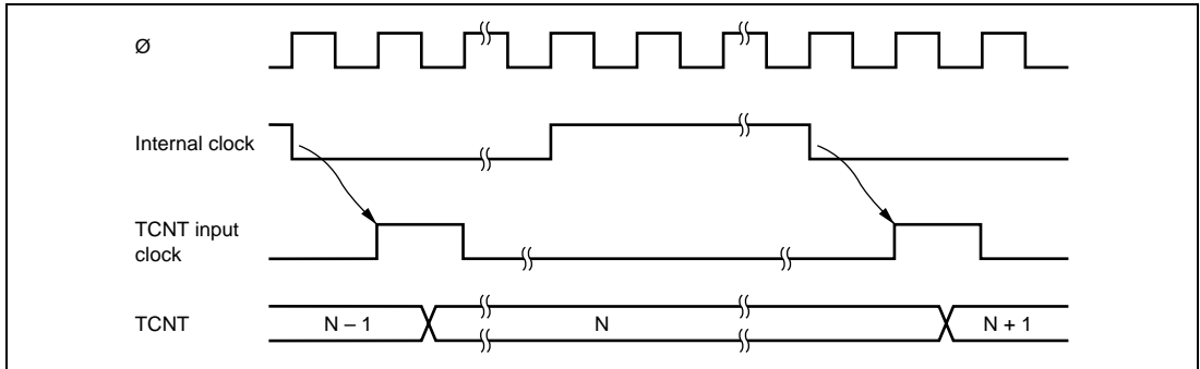
Figure 12.4 Count Timing for Internal Clock Input
