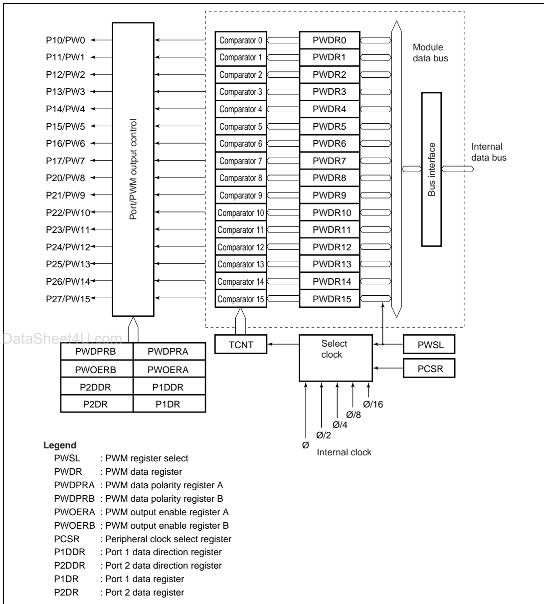
Figure 9.1 Block Diagram of PWM Timer
