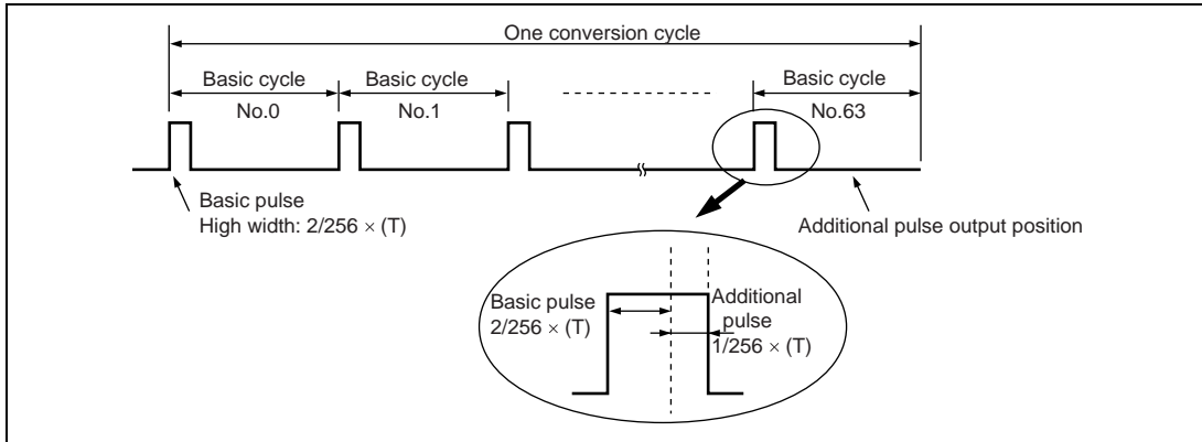
Figure 10.6 Output Waveform when DADR = H'0207 ( OS = 1 )
