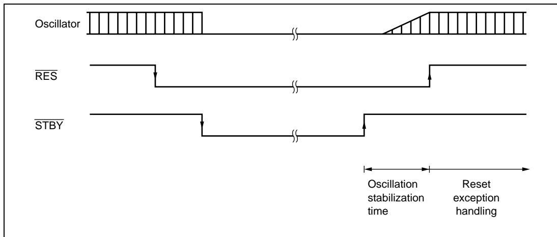
Figure 26.4 Hardware Standby Mode Timing
