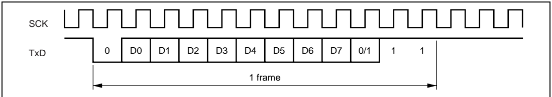
Figure 15.4 Relation between Output Clock and Transmit Data Phase (Asynchronous Mode)
