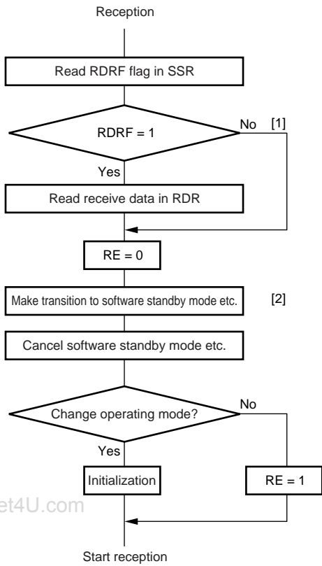
Figure 15.27 Sample Flowchart for Mode Transition during Reception
