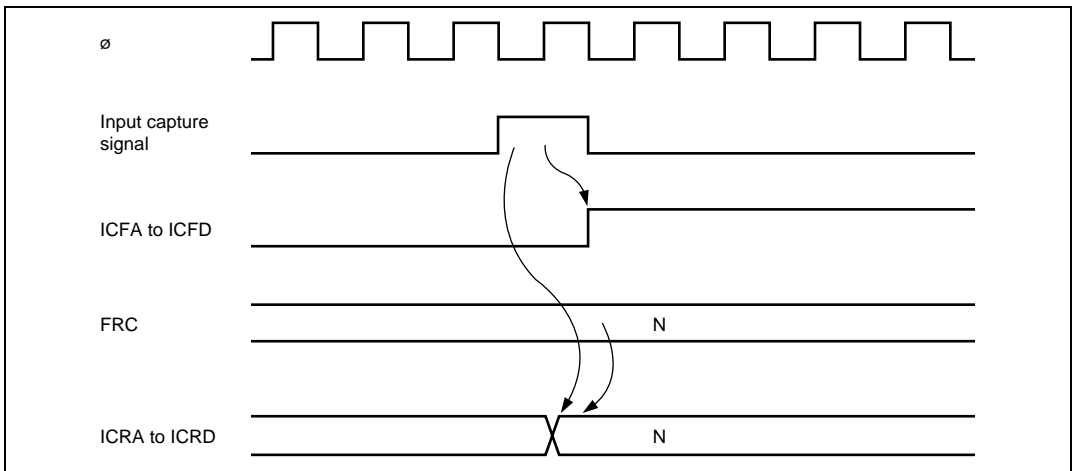
Figure 11.11 Timing of Input Capture Flag (ICFA, ICFB, ICFC, or ICFD) Setting
