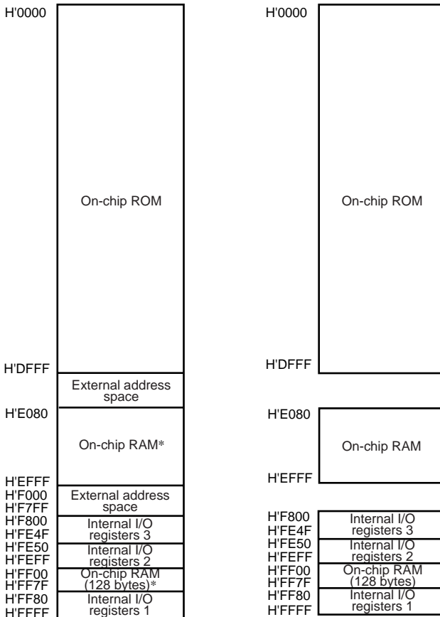
Figure 3.4 Address Map for H8S/2141B and H8S/2161B (2)
