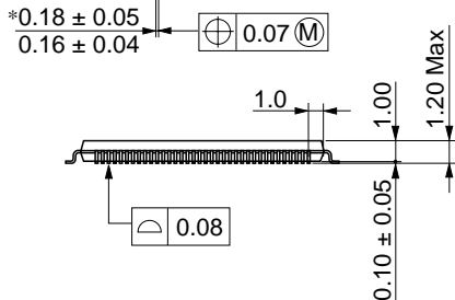
Figure C.3 Package Dimensions (TFP-144)
