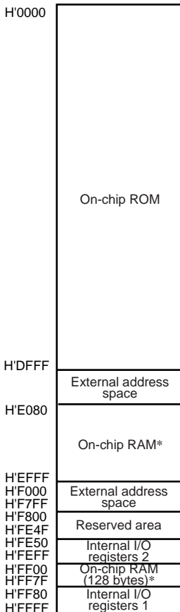
Figure 3.8 Address Map for H8S/2148B (2)
