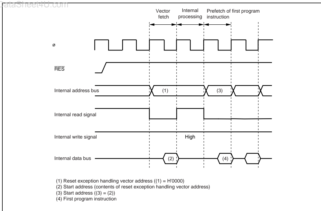
Figure 4.1 Reset Sequence (Mode 3)
