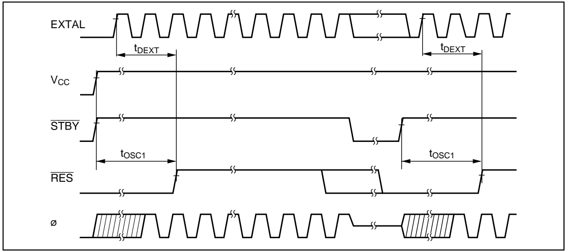
Figure 28.7 Oscillation Settling Timing
