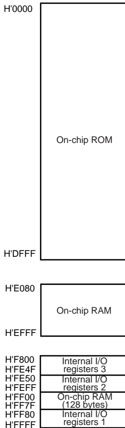
Figure 3.2 Address Map for H8S/2140B and H8S/2160B (2)
