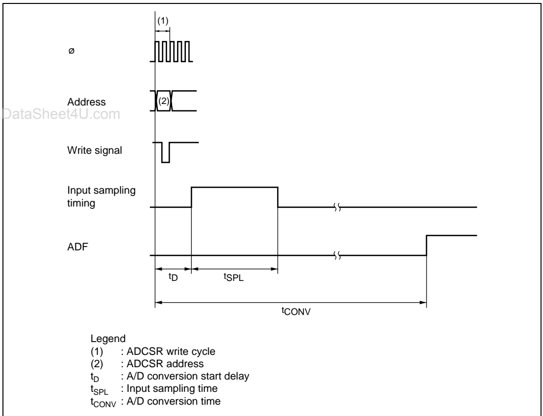
Figure 21.3 A/D Conversion Timing
