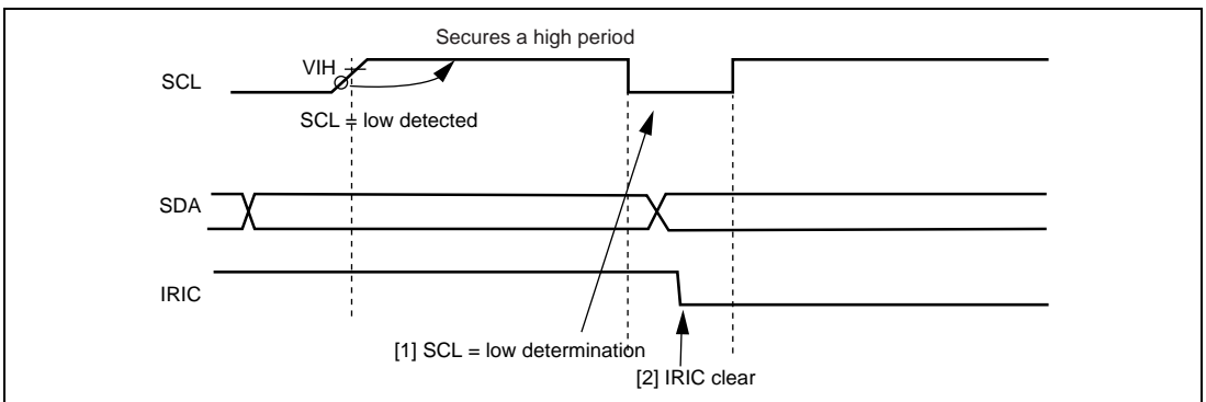
Figure 16.33 IRIC Flag Clearing Timing When WAIT = 1
