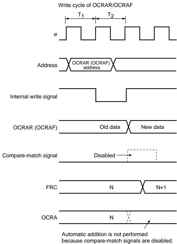
Figure 11.20 Conflict between OCRAR/OCRAF Write and Compare-Match (When Automatic Addition Function is Used)
