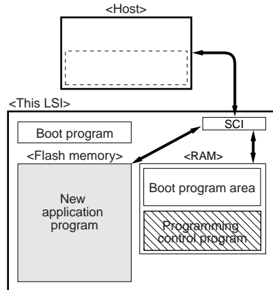
Figure 23.3 Boot Mode
