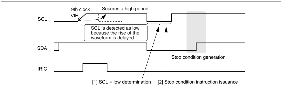
Figure 16.32 Stop Condition Issuance Timing
