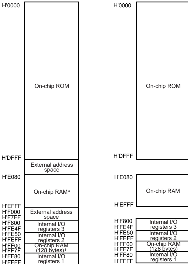
Figure 3.6 Address Map for H8S/2145BV (2)
