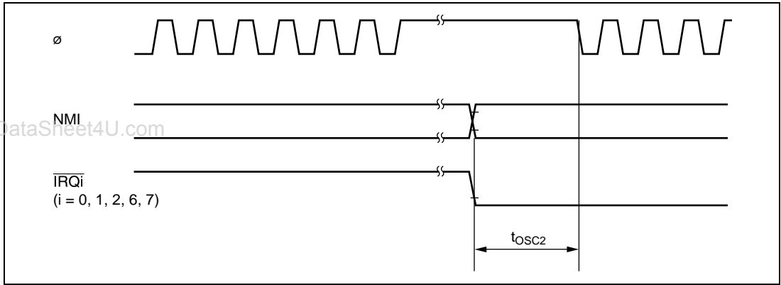
Figure 28.8 Oscillation Settling Timing (Exiting Software Standby Mode)
