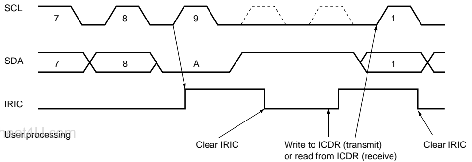
Figure 16.26 IRIC Setting Timing and SCL Control (1)
