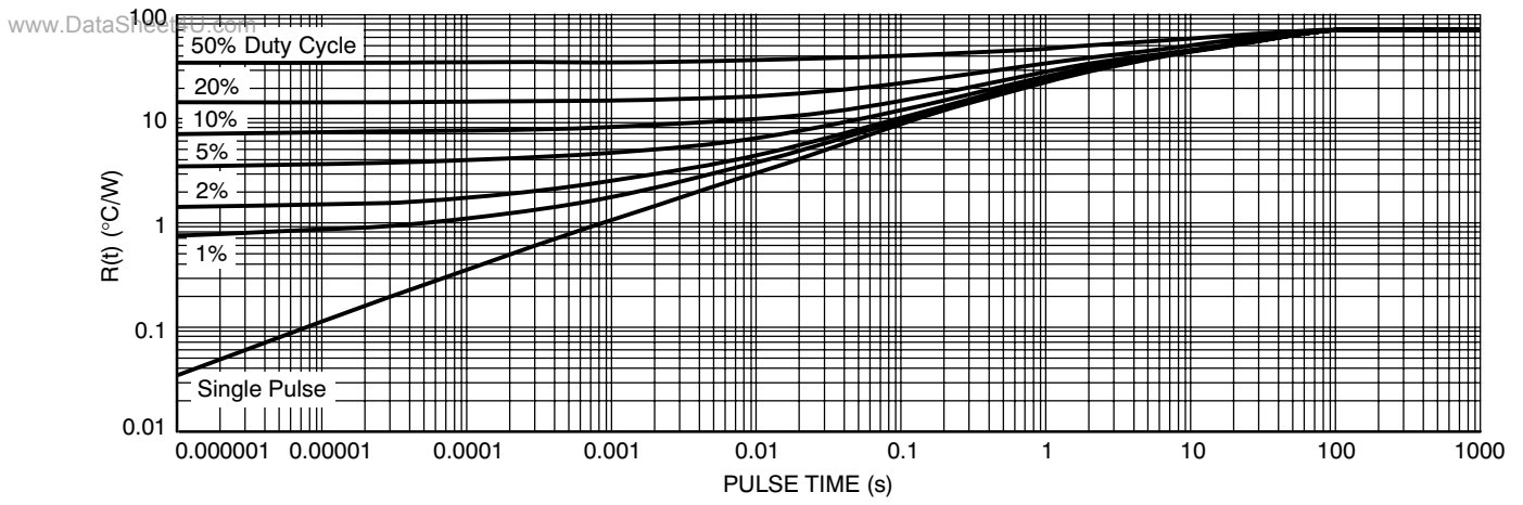
Figure 10. Thermal Response, Junction-to-Ambient
