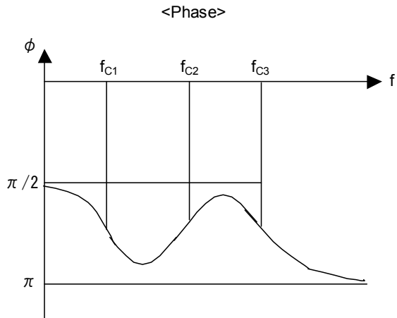
Fig.71 (Fig.58) Frequency – Phase Characteristics
