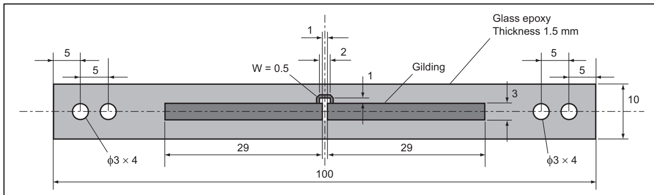
Figure 1 Evaluation Antenna
