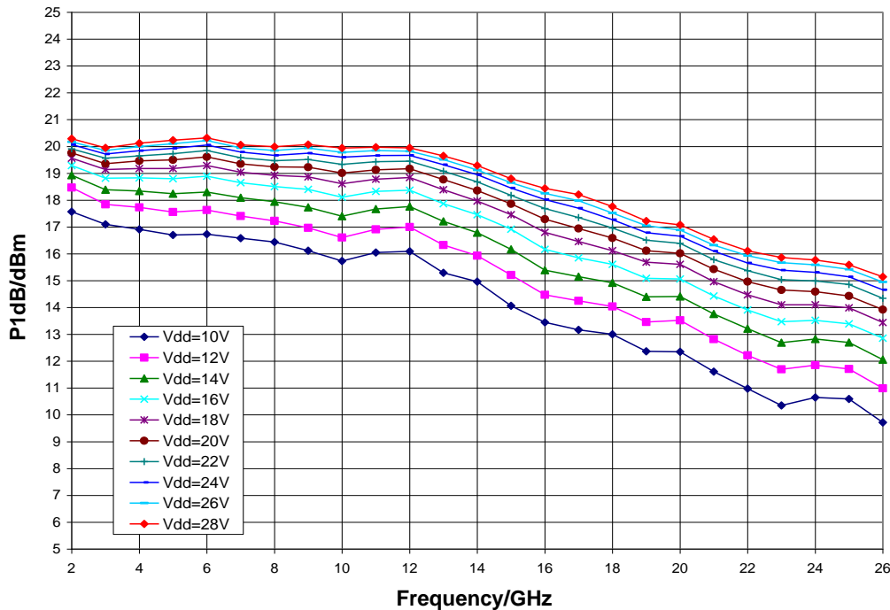
P1dB vs. V_{dd} , V_{gg} = -3\text{ V} , T_A = 25^\circ\text{C}
