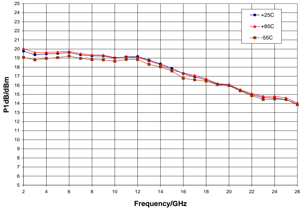
P1dB vs. Temperature, V_{dd} = 20\text{ V} , V_{gg} = -3\text{ V}
