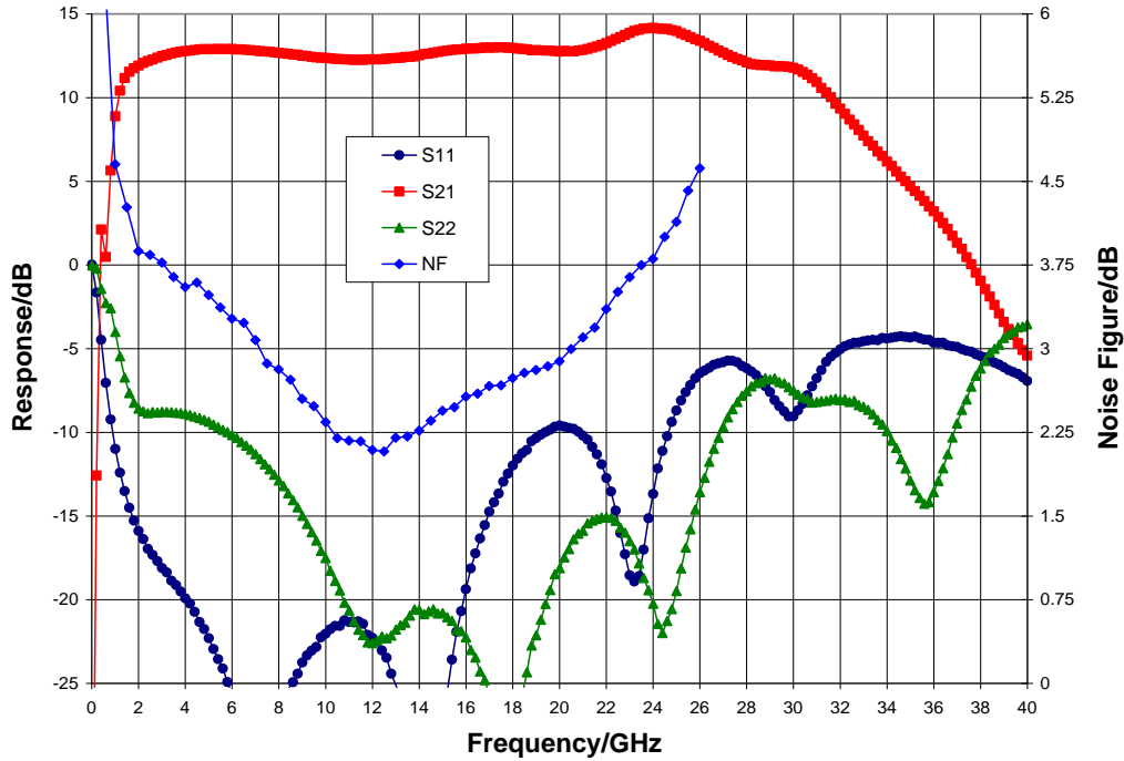
Broadband Performance, V_{dd} = 20\text{ V} , V_{gg} = -3\text{ V} , I_{dd} = 100\text{ mA} , T_A = 25^\circ\text{ C}
