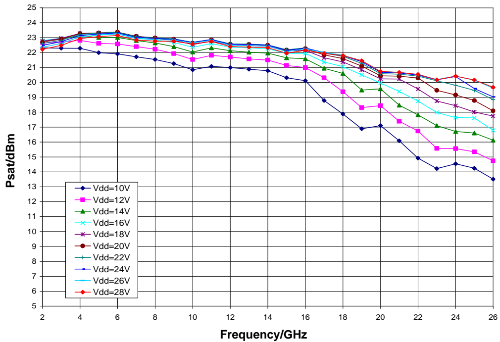
Psat vs. V_{dd} , V_{gg} = -3\text{ V} , T_A = 25^\circ\text{ C}
