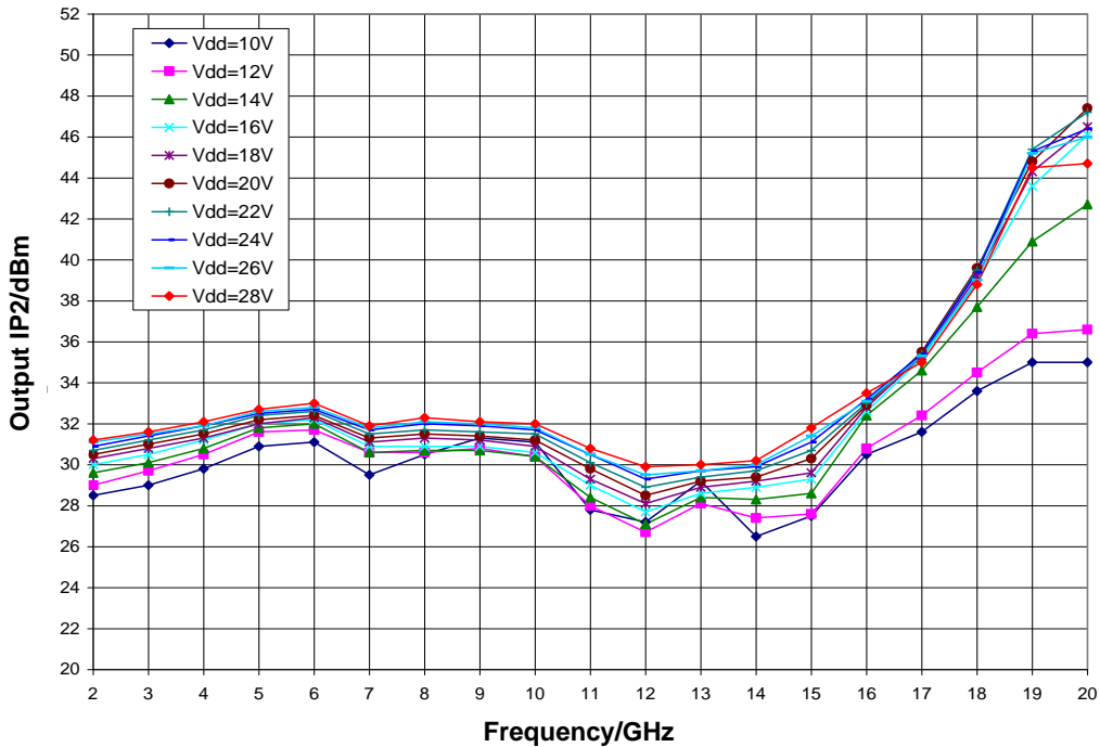
Output IP2 vs. V_{dd} , V_{gg} = -3\text{ V} , T_A = 25^\circ\text{ C}
