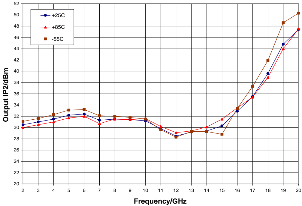
Output IP2 vs. Temperature, V_{dd} = 20\text{ V} , V_{gg} = -3\text{ V}
