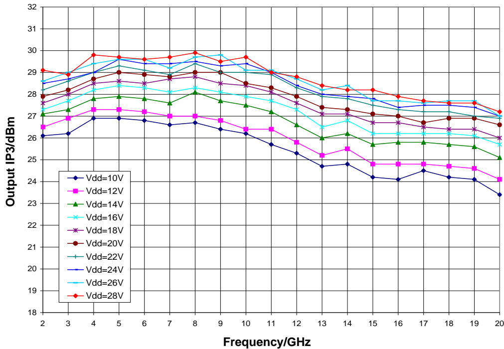
Output IP3 vs. V_{dd} , V_{gg} = -3\text{ V} , T_A = 25^\circ\text{ C}
