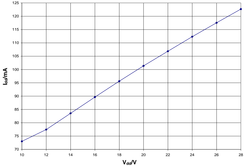
Drain Current vs. Drain Voltage, V_{gg} = -3\text{ V} , T_A = 25^\circ\text{ C}
