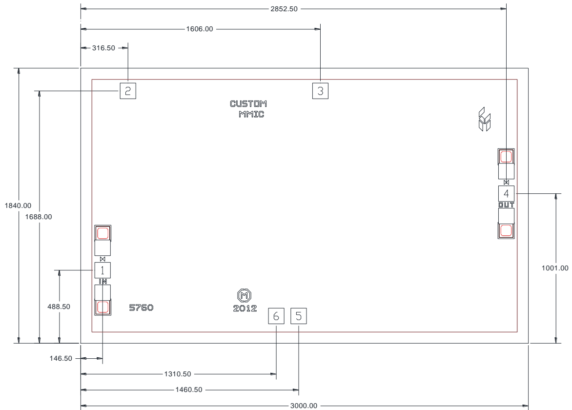
Die Outline (all dimensions in microns)
