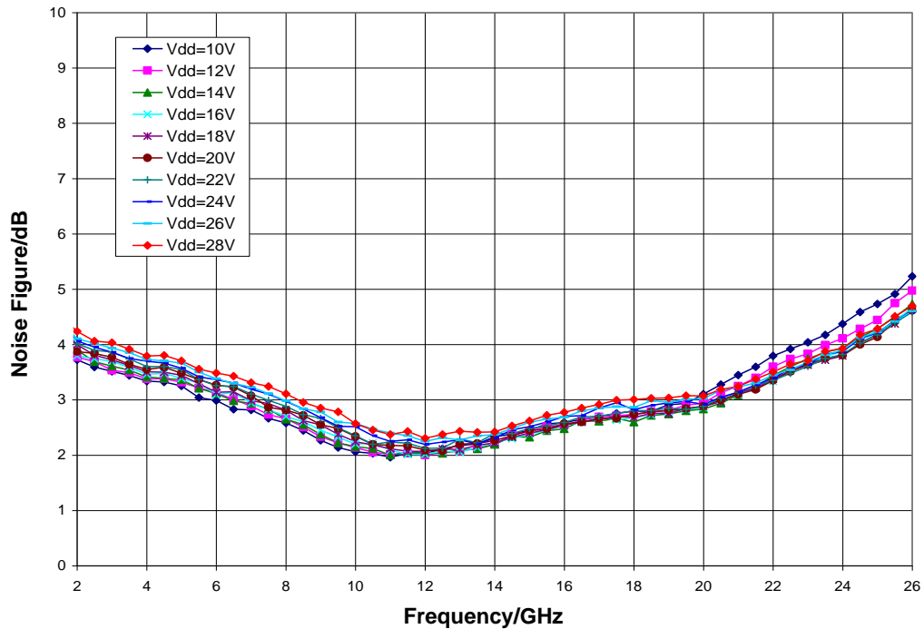
Noise Figure vs. V_{dd} , V_{gg} = -3\text{ V} , T_A = 25^\circ\text{ C}
