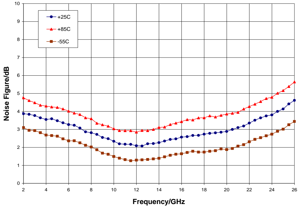
Noise Figure vs. Temperature, V_{dd} = 20\text{ V} , V_{gg} = -3\text{ V}
