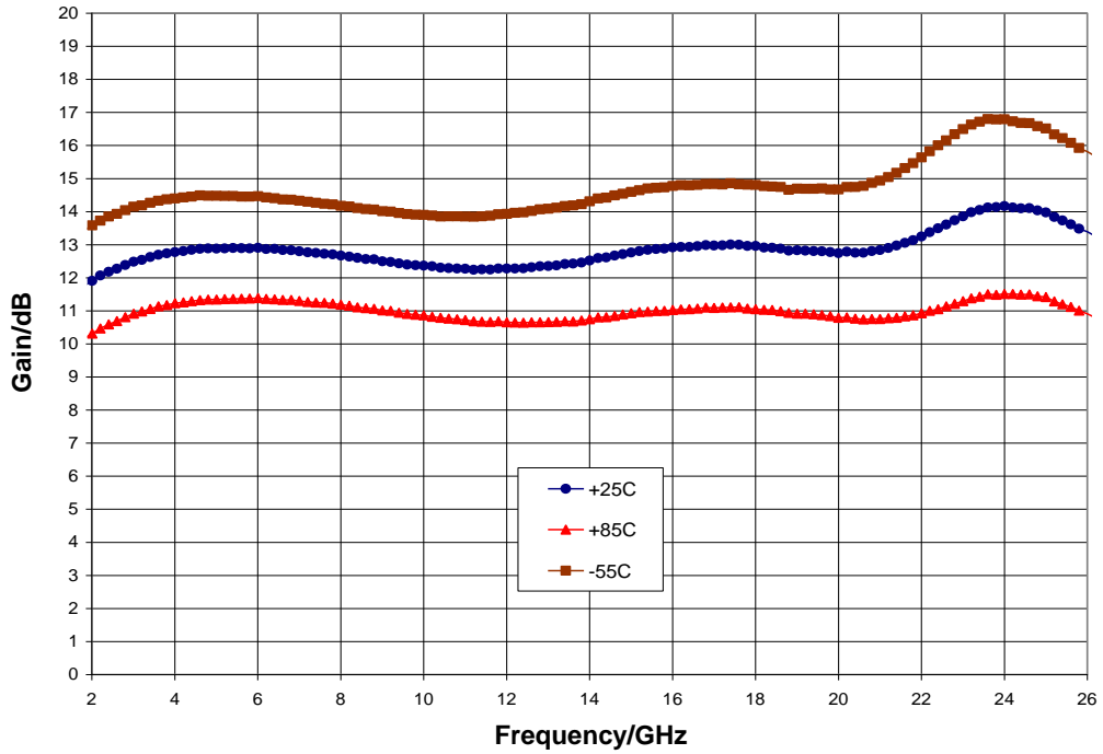
Gain vs. Temperature, V_{dd} = 20\text{ V} , V_{gg} = -3\text{ V}
