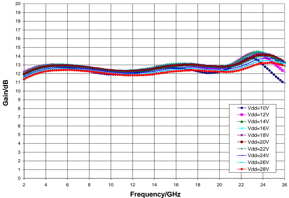
Gain vs. V_{dd} , V_{gg} = -3\text{ V} , T_A = 25^\circ\text{ C}
