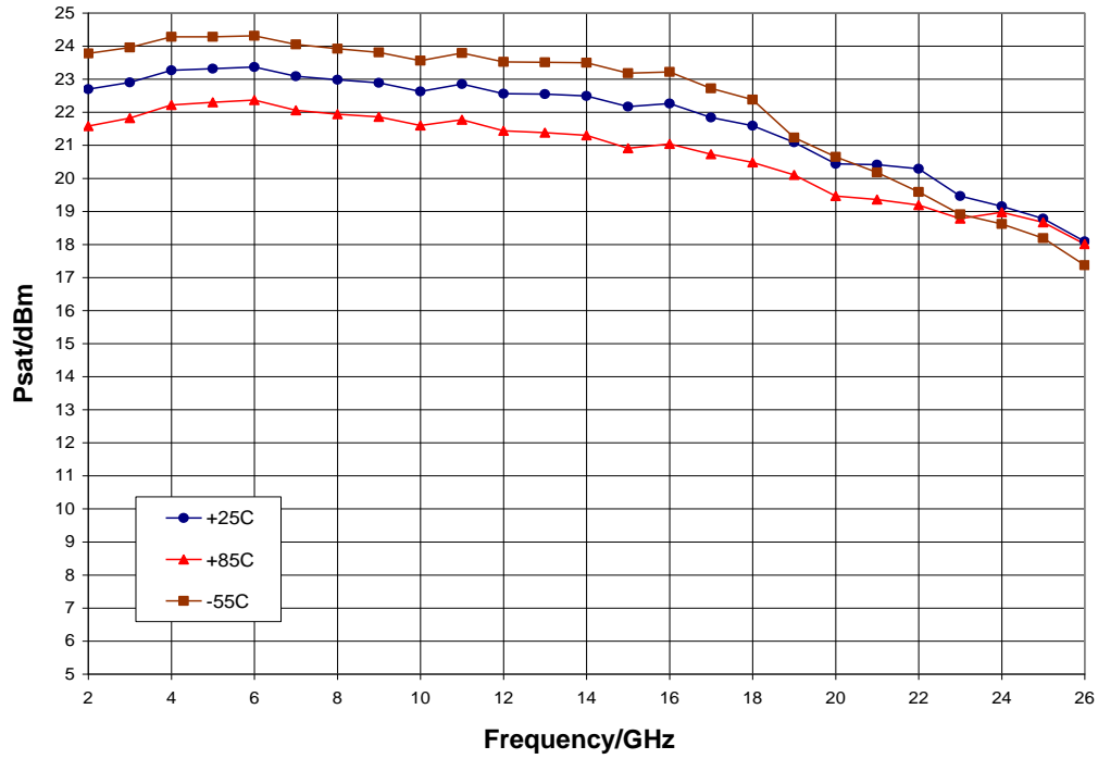
Psat vs. Temperature, V_{dd} = 20\text{ V} , V_{gg} = -3\text{ V}
