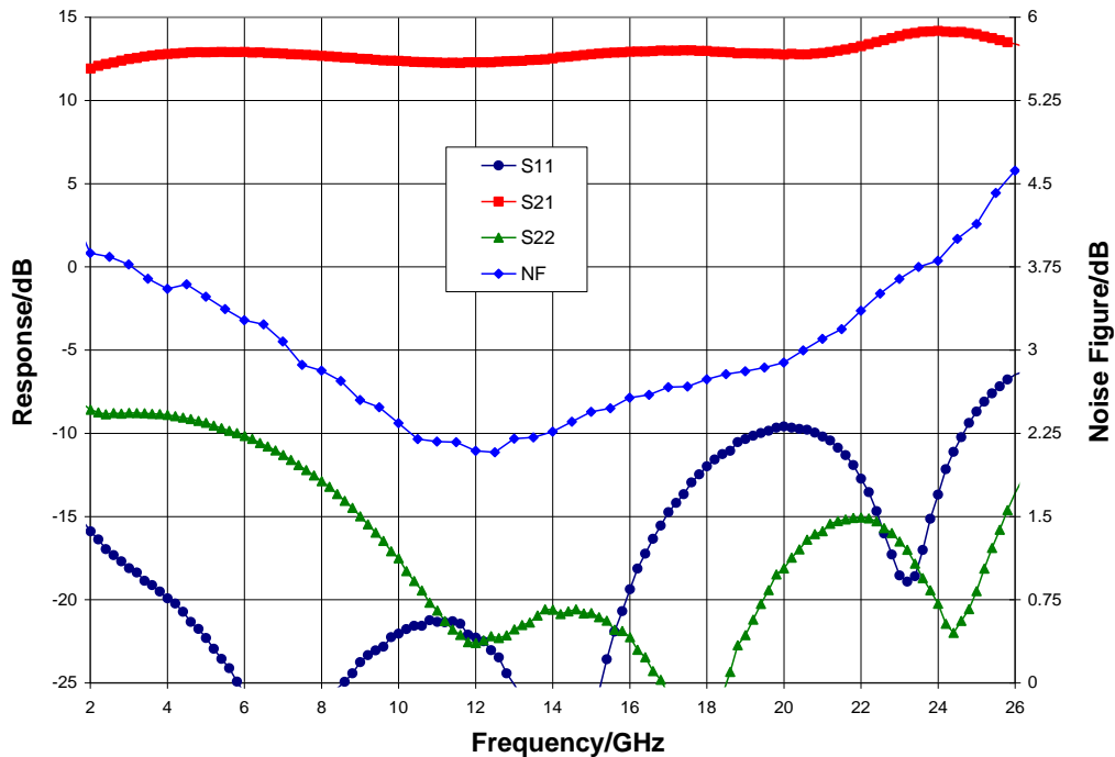
Narrow-band Performance, V_{dd} = 20\text{ V} , V_{gg} = -3\text{ V} , I_{dd} = 100\text{ mA} , T_A = 25^\circ\text{ C}
