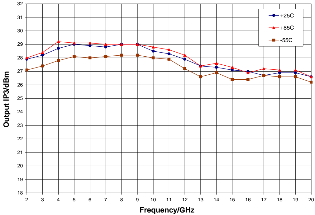
Output IP3 vs. Temperature, V_{dd} = 20\text{ V} , V_{gg} = -3\text{ V}
