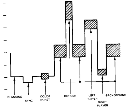
Fig. 1 COMPOSITE VIDEO OUTPUT
