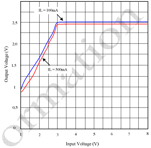
Dropout Characteristics
