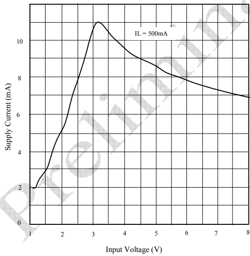
Supply Current vs. Input Voltage
