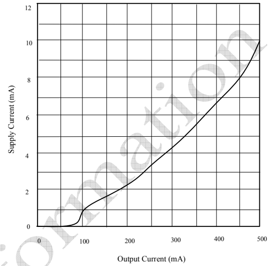
Supply Current vs. Load Current
