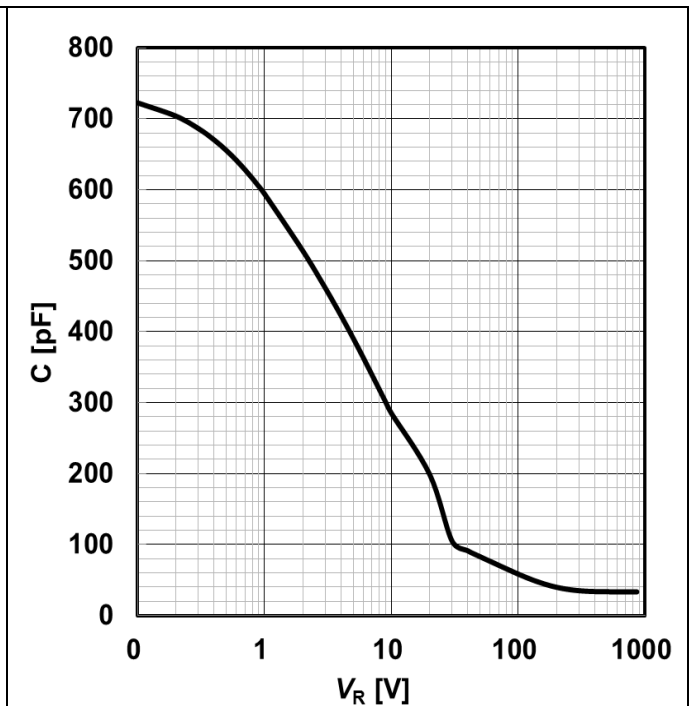
C = f(V_R); T_j = 25\text{ °C}; f = 1\text{ MHz}
