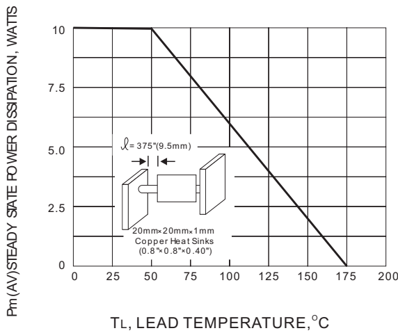
Fig.5 STEADY STATE POWER DERATING
