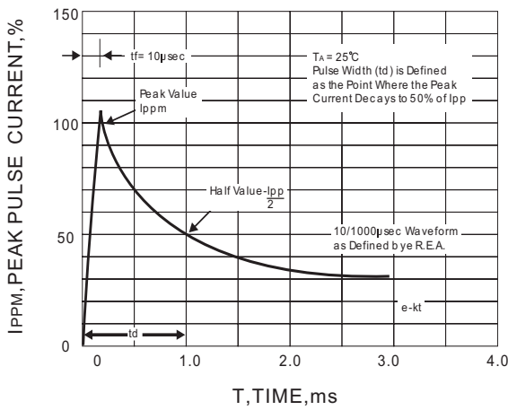
Fig.3 PULSE WAVEFORM
