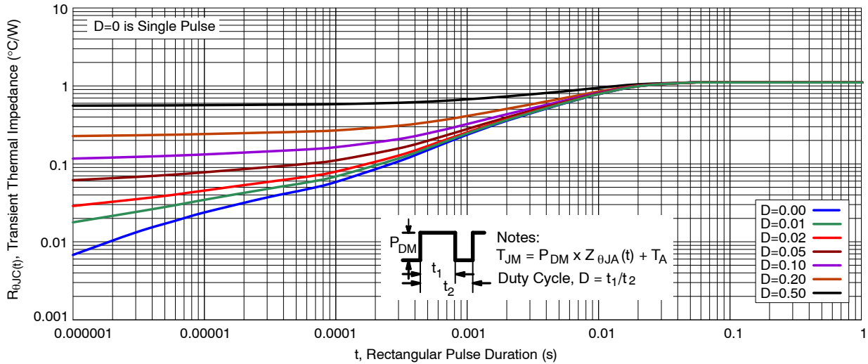
Figure 14. Thermal Response
