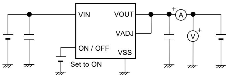
Figure 13 Test Circuit 9
