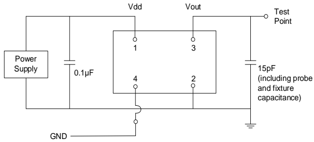
Figure 2. Test Circuit [10]
