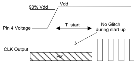
Figure 4. Startup Timing [11]
