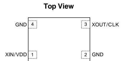
Figure 1. Pin Assignments
