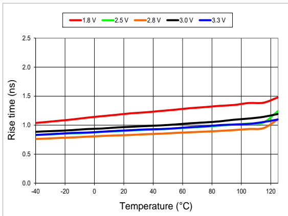
Figure 9. 20%-80% Rise Time vs Temperature
