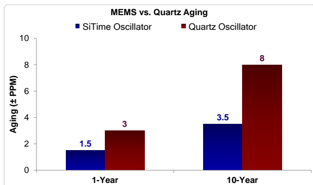
Figure 2. Aging Comparison [2]
