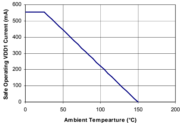
Figure 2. Thermal Derating Curve, Dependence of Safety Limiting Values on Case Temperature, per DIN EN 60747-5-2
