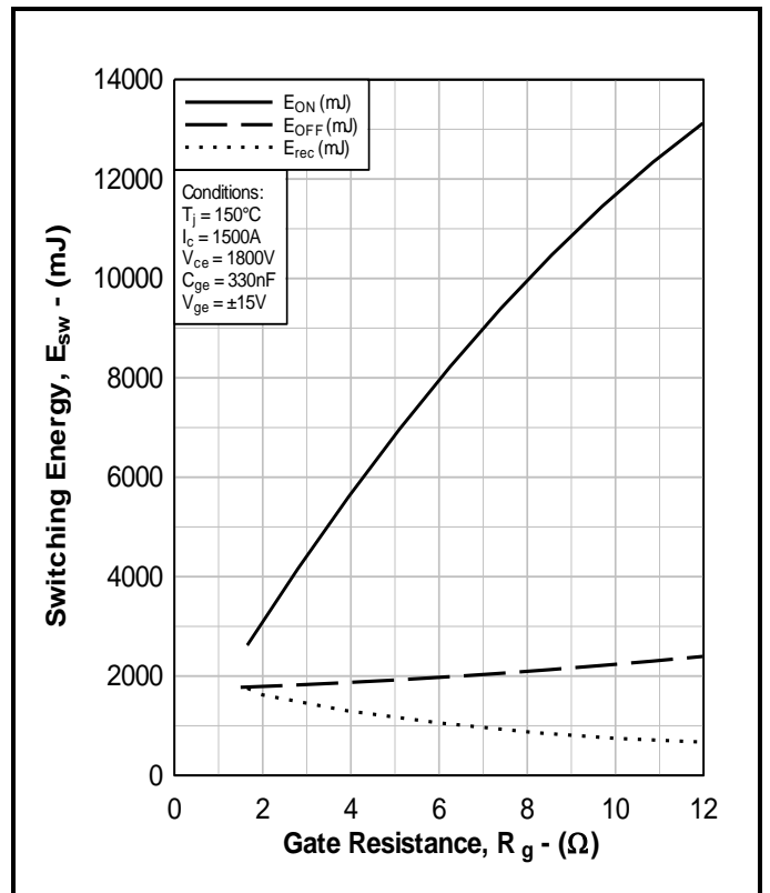
Fig. 6 Typical switching energy vs gate resistance
