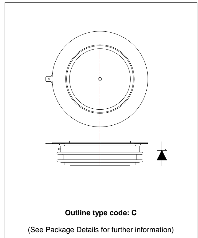
Fig. 1 Package outline
