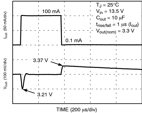
Figure 22. Load Transients
