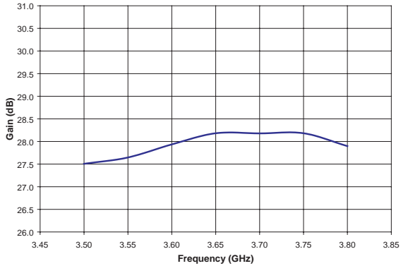
Figure 4: Gain vs. Frequency ( T_C = +25\text{ }^\circ\text{C} , V_{CC} = +6.0\text{ V} , V_{BIAS} = +3.0\text{ V} , P_{OUT} = +24\text{ dBm} , 54 Mbps OFDM Modulation)
