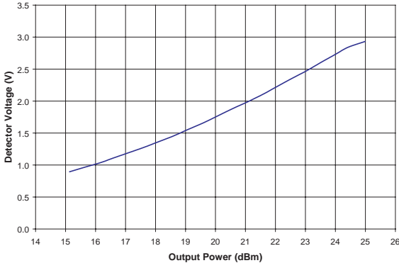
Figure 7: Detector Voltage vs. Output Power ( T_C = +25\text{ }^\circ\text{C} , V_{CC} = +6.0\text{ V} , V_{BIAS} = +3.0\text{ V} , f = 3.7\text{ GHz} , 54 Mbps OFDM Modulation)
