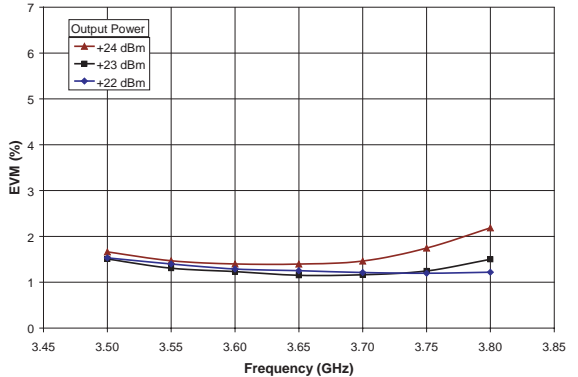
Figure 6: Uncorrected EVM vs. Frequency ( T_C = +25\text{ }^\circ\text{C} , V_{CC} = +6.0\text{ V} , V_{BIAS} = +3.0\text{ V} , 54 Mbps OFDM Modulation, system EVM Approx. 0.8 %)
