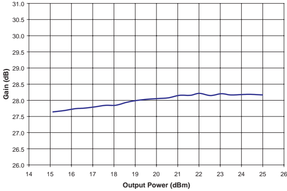
Figure 3: Gain vs. Output Power ( T_C = +25\text{ }^\circ\text{C} , V_{CC} = +6.0\text{ V} , V_{BIAS} = +3.0\text{ V} , f = 3.7\text{ GHz} , 54 Mbps OFDM Modulation)
