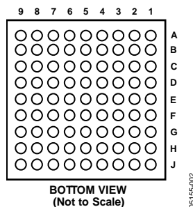
Figure 3. Pin Configuration
