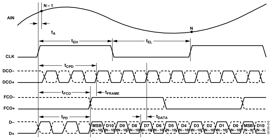
Figure 2. Timing Diagram
