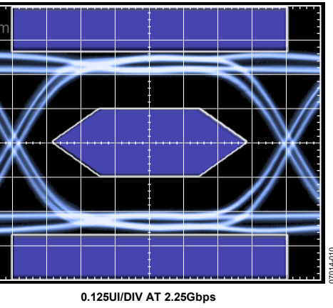
Figure 10. Tx Eye Diagram at TP2, PE = 2 dB
