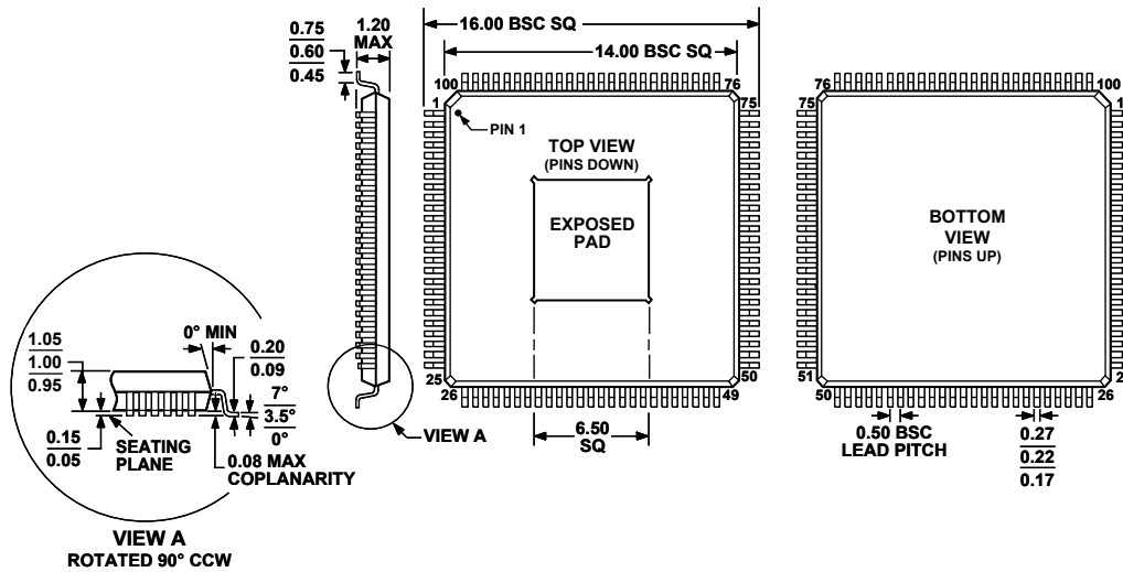
COMPLIANT TO JEDEC STANDARDS MS-026-AED-HD Figure 19. 100-Lead Thin Quad Flat Package, Exposed Pad [TQFP_EP] (SV-100-2) Dimensions shown in millimeters
