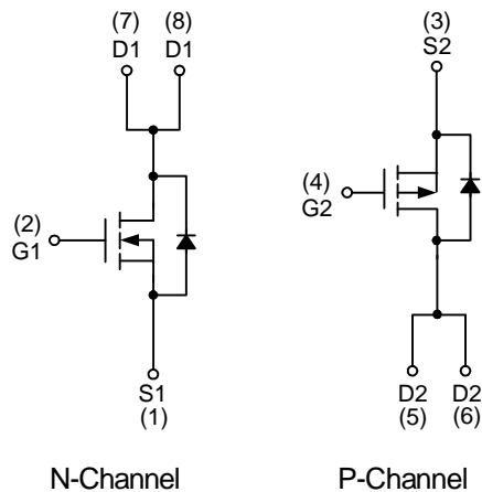
Top View of SOP – 8
