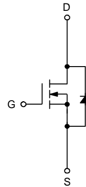
N-Channel MOSFET
