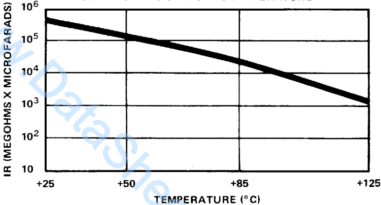
INSULATION RESISTANCE VS TEMPERATURE
