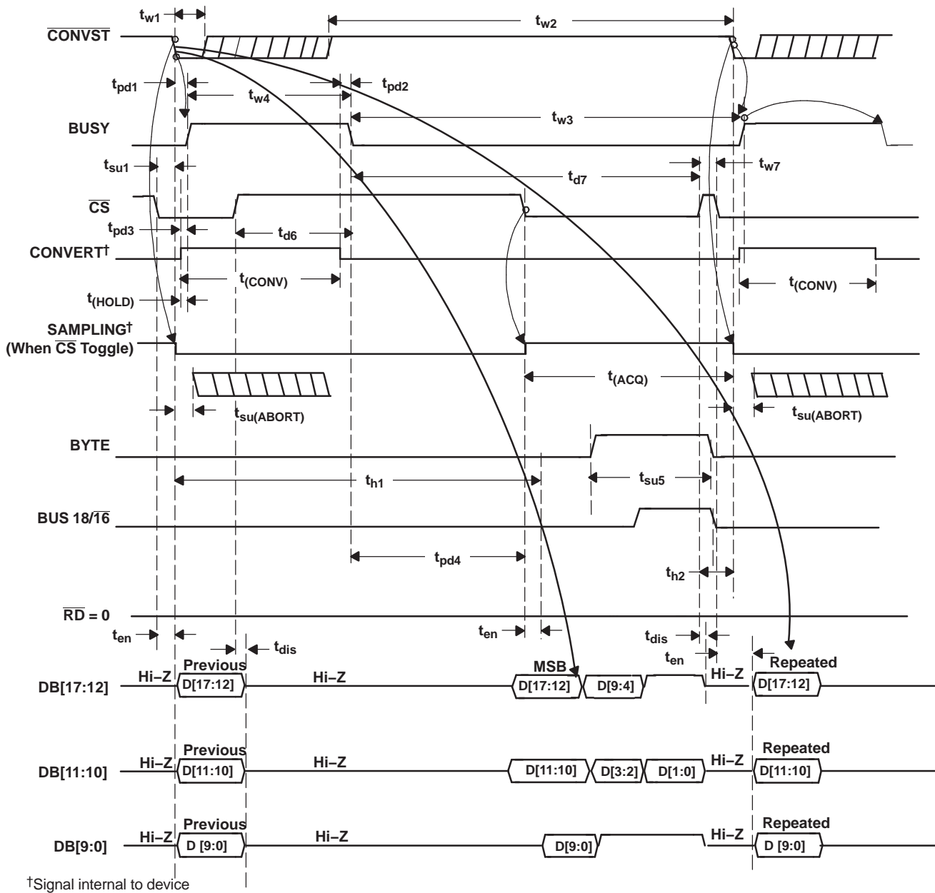
Figure 31. Timing for Conversion and Acquisition Cycles With \overline{\text{CS}} Toggling, \overline{\text{RD}} Tied to BDGND
