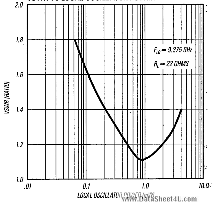
VSWR VS LOCAL OSCILLATOR POWER
