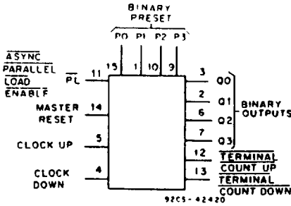
FUNCTIONAL DIAGRAM
