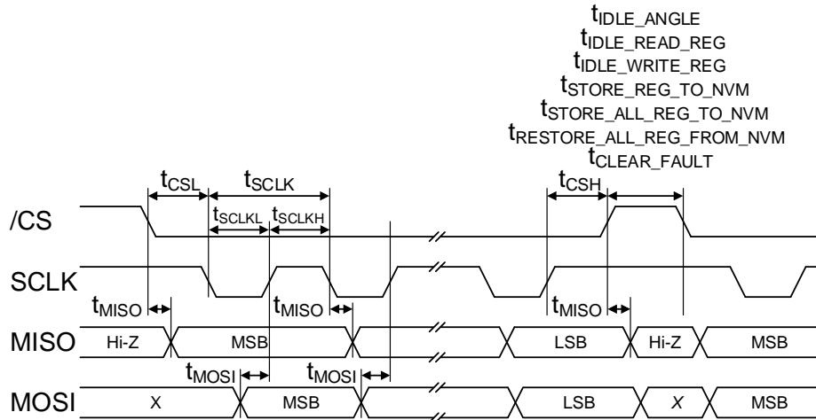
Figure 12: SPI Timing Diagram (Mode 3)
