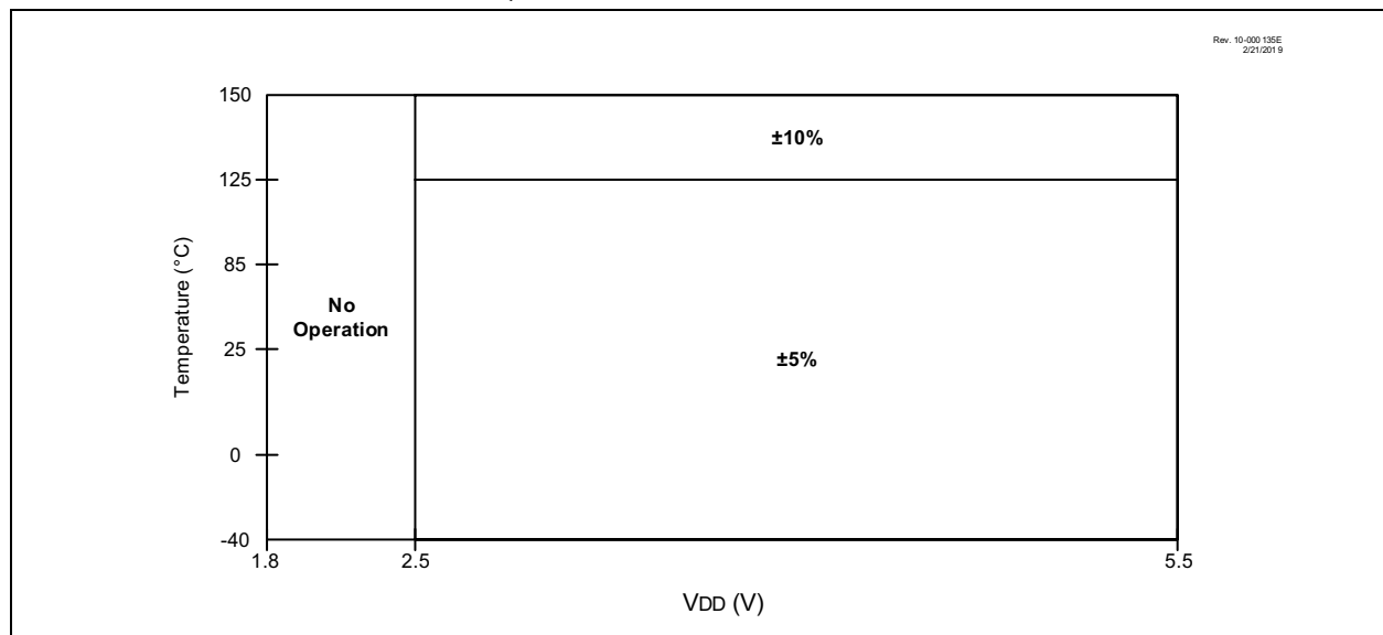
FIGURE 3-2: HFINTOSC FREQUENCY ACCURACY OVER V_{\text{DD}} AND TEMPERATURE
