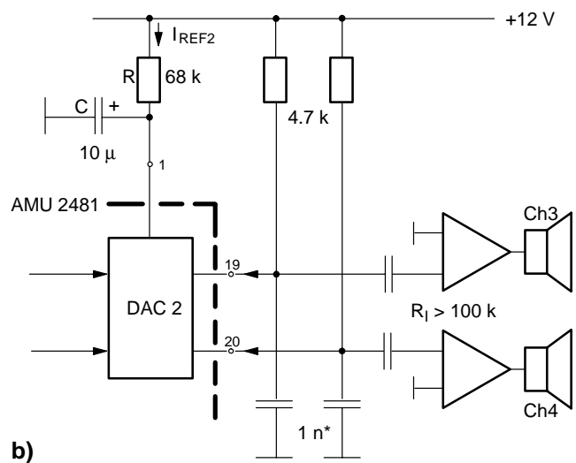
Fig. 2–3: DAC application diagrams a) DAC 1 Interface b) DAC 2 Interface
