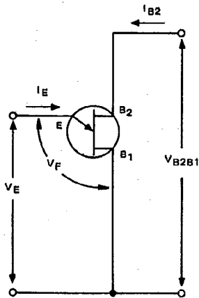
FIGURE 1 UNIUNJUNCTION TRANSISTOR SYMBOL AND NOMENCLATURE
