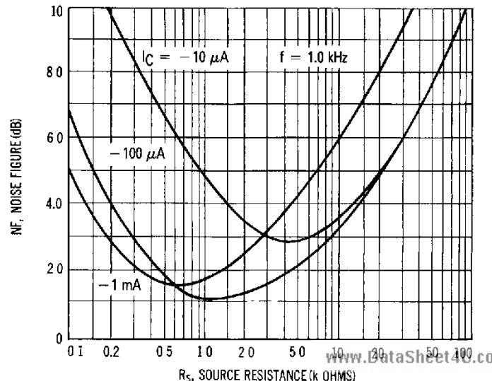
FIGURE 6 – SOURCE RESISTANCE EFFECTS
