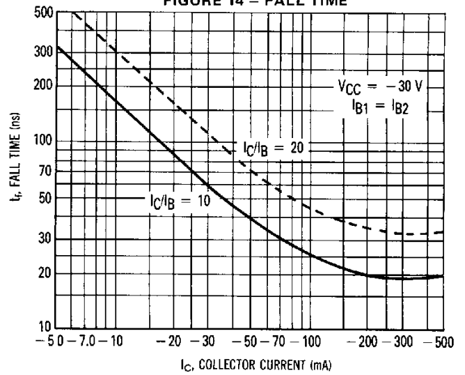
FIGURE 14 – FALL TIME
