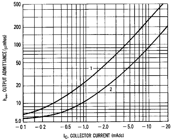
FIGURE 10 – OUTPUT ADMITTANCE
