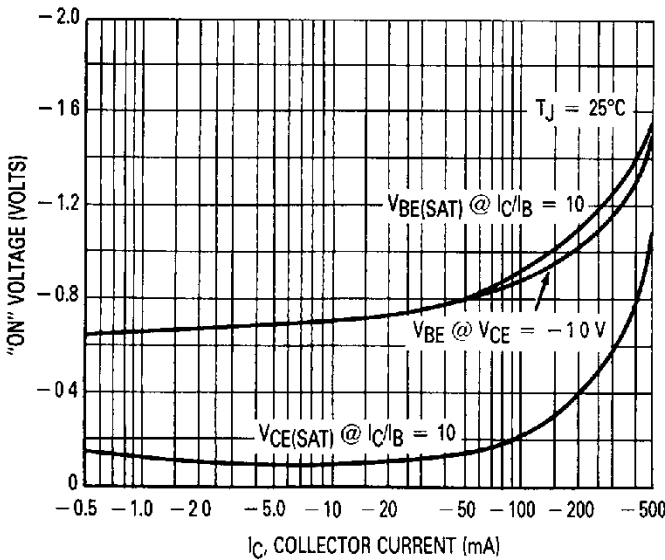
FIGURE 3 – "ON" VOLTAGES
