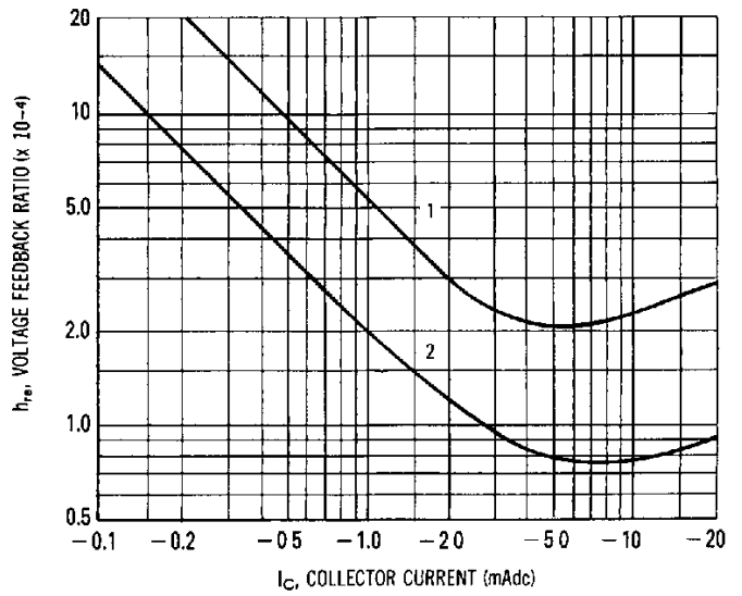
FIGURE 8 – VOLTAGE FEEDBACK RATIO
