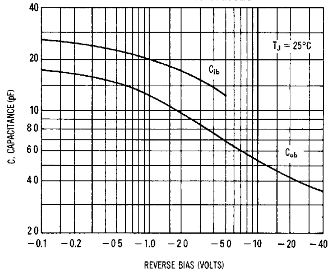
FIGURE 17 – CAPACITANCES
