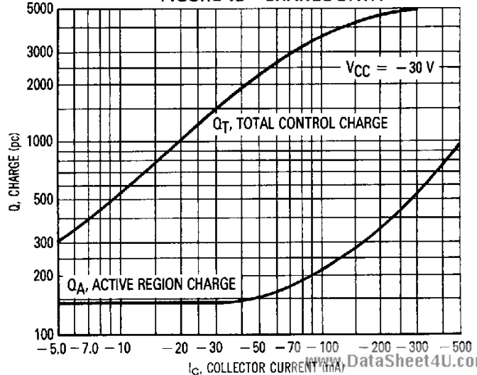
FIGURE 12 – CHARGE DATA
