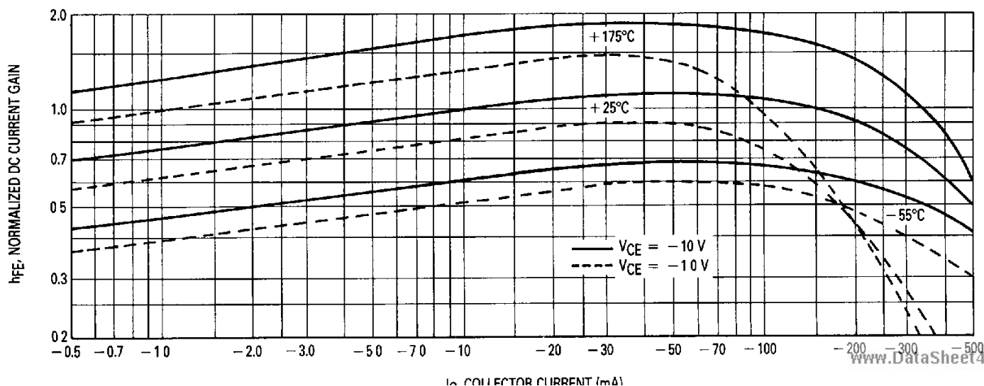
FIGURE 1 – NORMALIZED DC CURRENT GAIN
