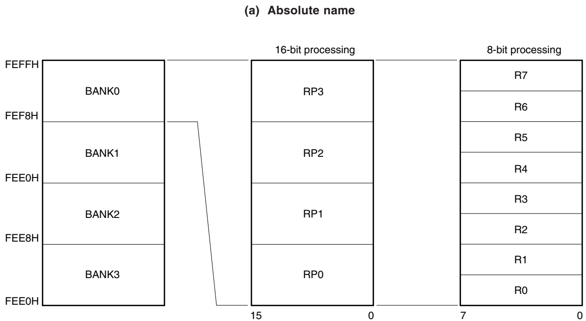
Figure 5-18. General-Purpose Register Configuration
