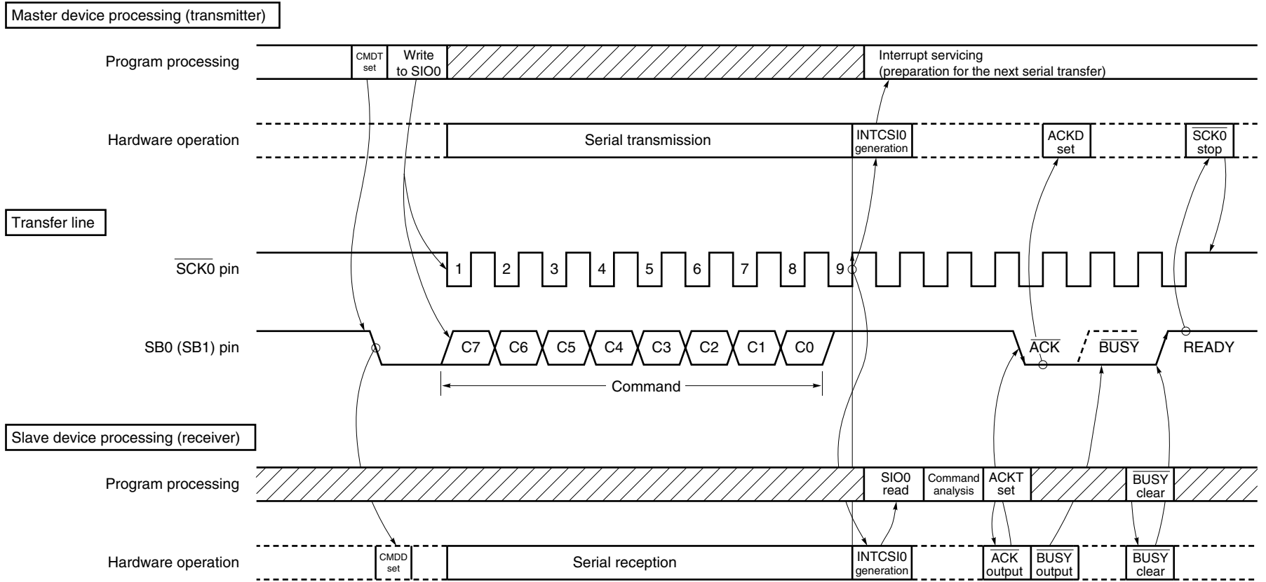
Figure 16-28. Command Transmission from Master Device to Slave Device
