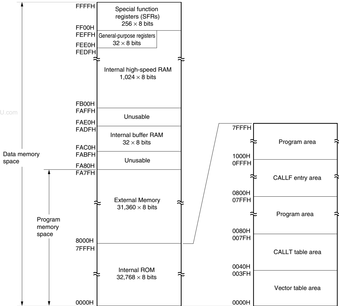
Figure 5-2. Memory Map ( \mu PD780054, 780054(A), 780054Y, 780054Y(A))
