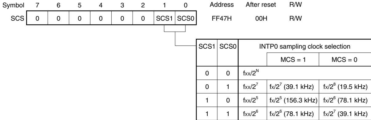
Figure 21-7. Format of Sampling Clock Select Register
