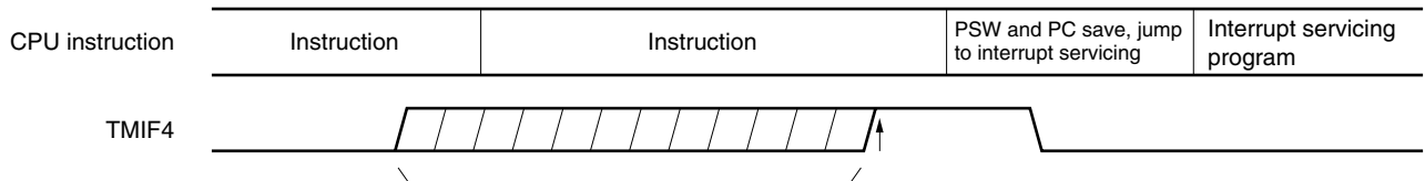
Figure 21-11. Non-Maskable Interrupt Request Acknowledgment Timing
