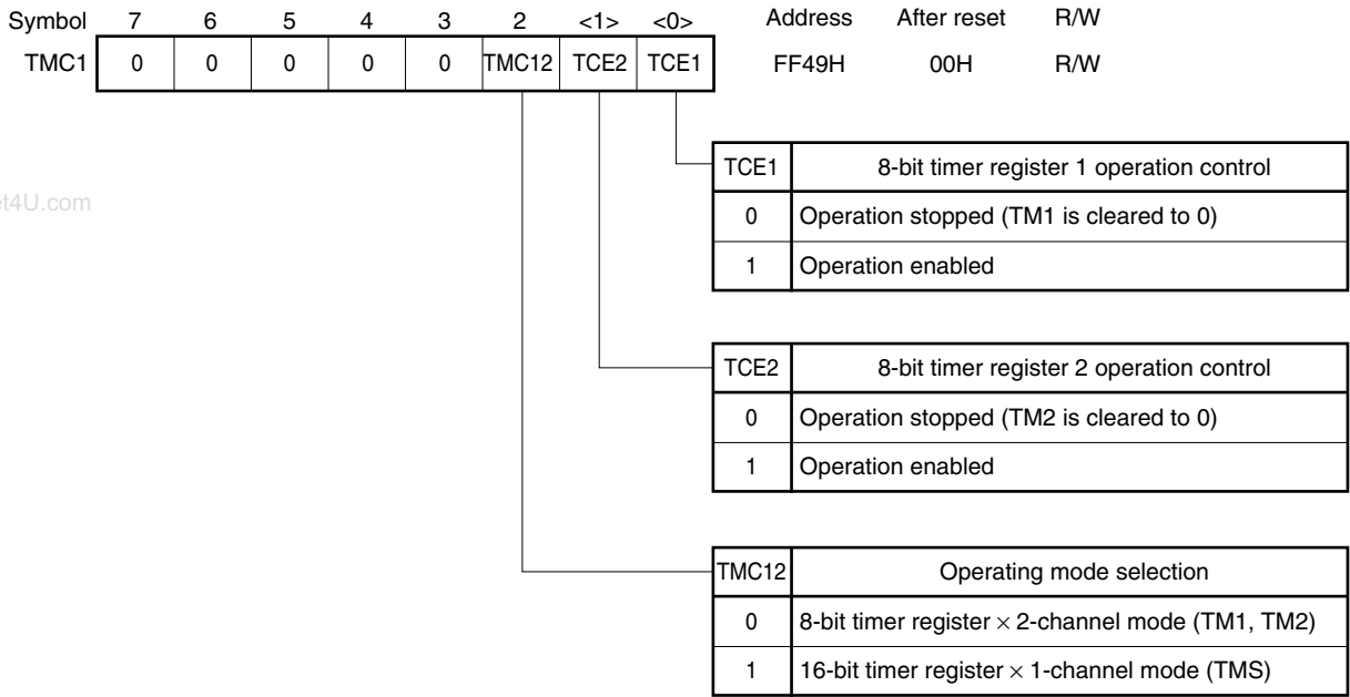
Figure 9-5. Format of 8-Bit Timer Mode Control Register 1
