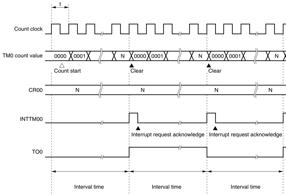
Figure 8-12. Interval Timer Operation Timings
