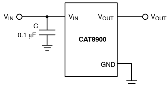
Figure 1. Application Circuit
