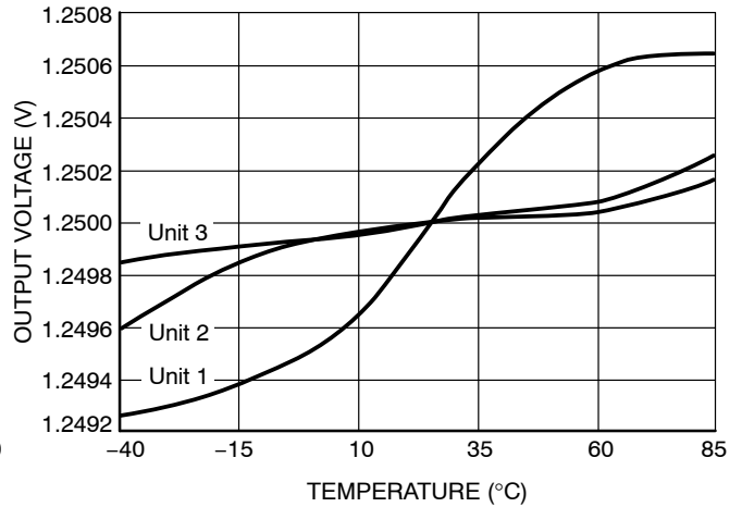
Figure 7. Output Voltage vs. Temperature Normalized
