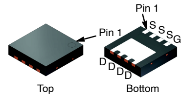
N-CHANNEL MOSFET
