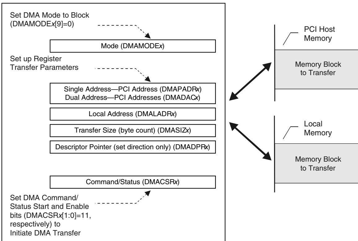
Figure 5-11. DMA Block Mode Initialization (Single Address or Dual Address PCI)
