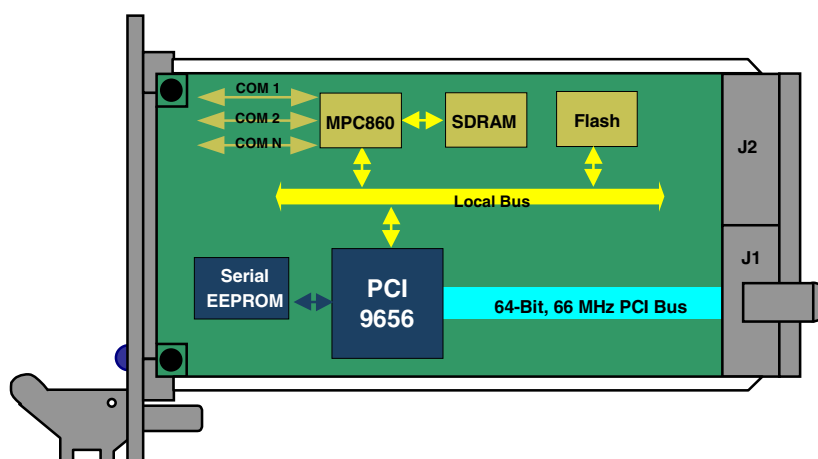
Figure 1-4. PCI 9656 CompactPCI Peripheral Card
