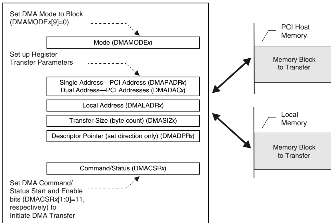
Figure 3-11. DMA Block Mode Initialization (Single Address or Dual Address PCI)
