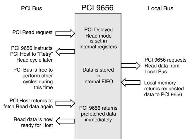
Figure 5-8. Direct Slave Delayed Read Mode
