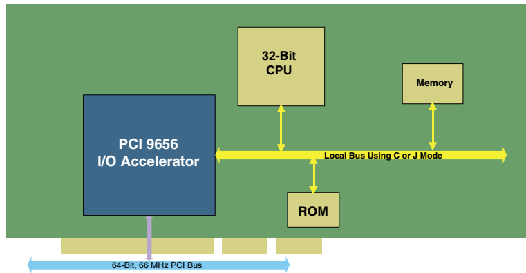
Figure 1-5. PCI 9656 PCI Adapter Card with C or J Mode Processor
