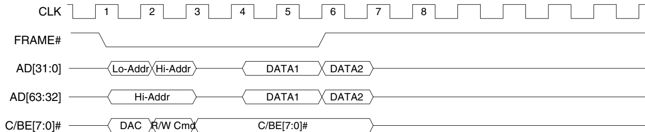
Figure 5-14. PCI Dual Address Cycle Timing
