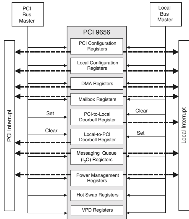
Figure 2-4. PCI 9656 Internal Register Access
