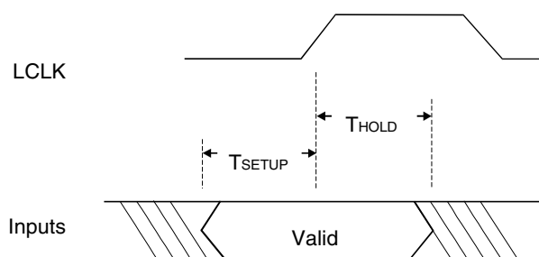
Figure 13-1. PCI 9656 Local Input Setup and Hold Timing
