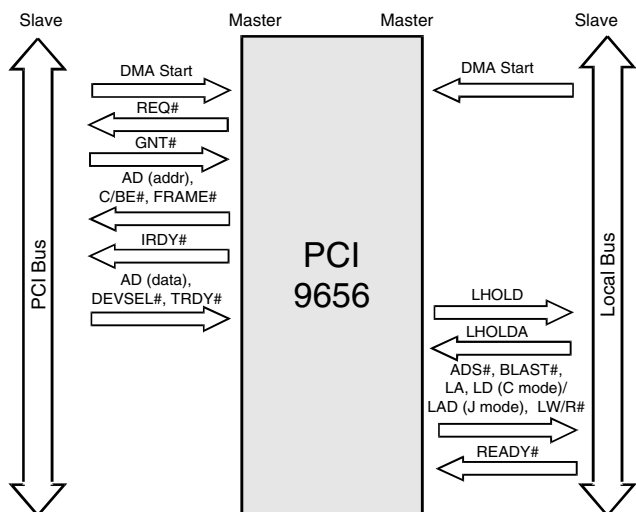
Figure 5-12. DMA, PCI-to-Local Bus
