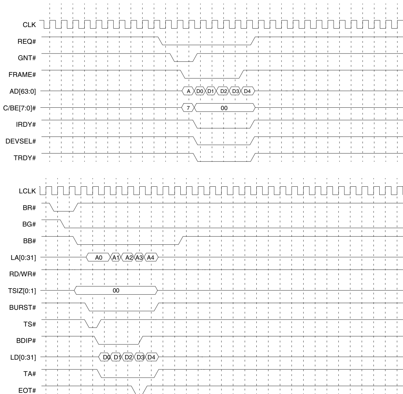
Timing Diagram 3-24. DMA Local-to-PCI, Continuous Burst Mode, with EOT# Assertion
