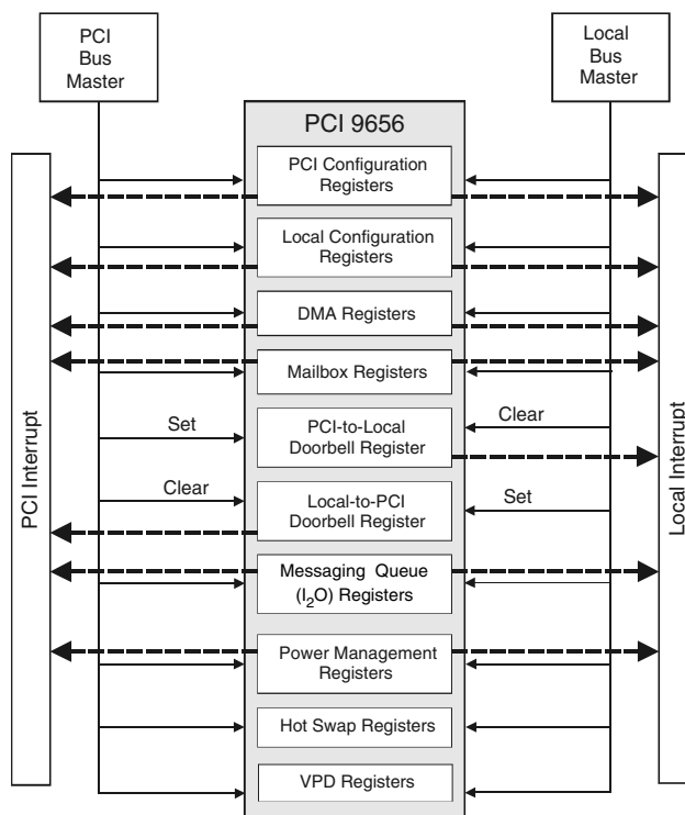
Figure 4-4. PCI 9656 Internal Register Access
