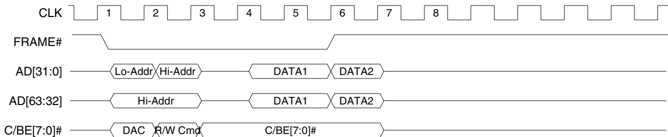
Figure 5-5. PCI Dual Address Cycle Timing
