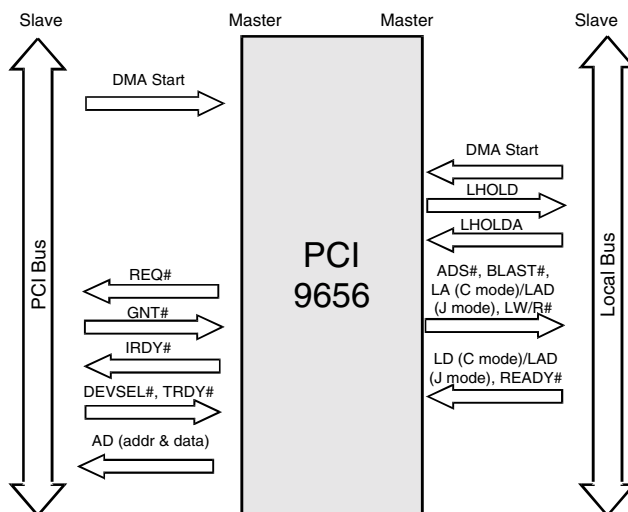
Figure 5-13. DMA, Local-to-PCI Bus
