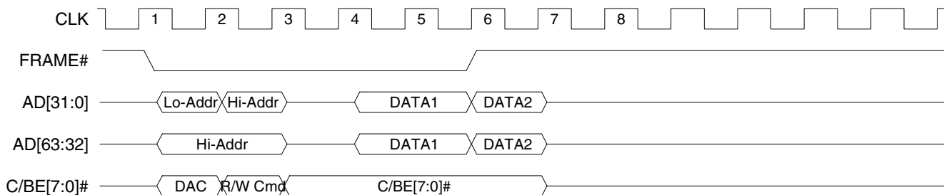
Figure 3-5. PCI Dual Address Cycle Timing
