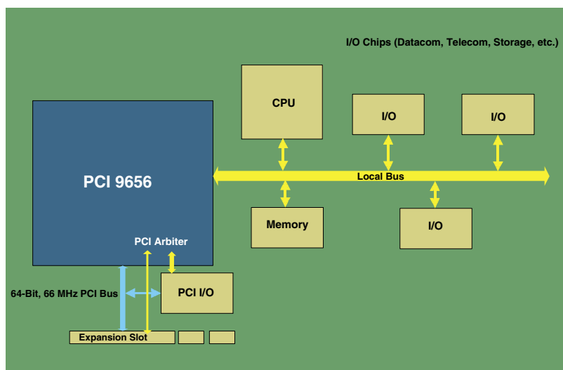
Figure 1-7. PCI 9656 Embedded Host System with Generic Host CPU
