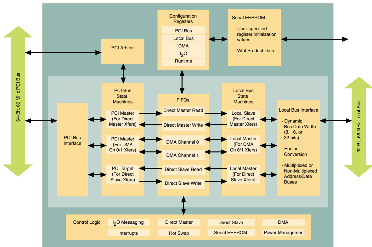
PCI 9656 Block Diagram
