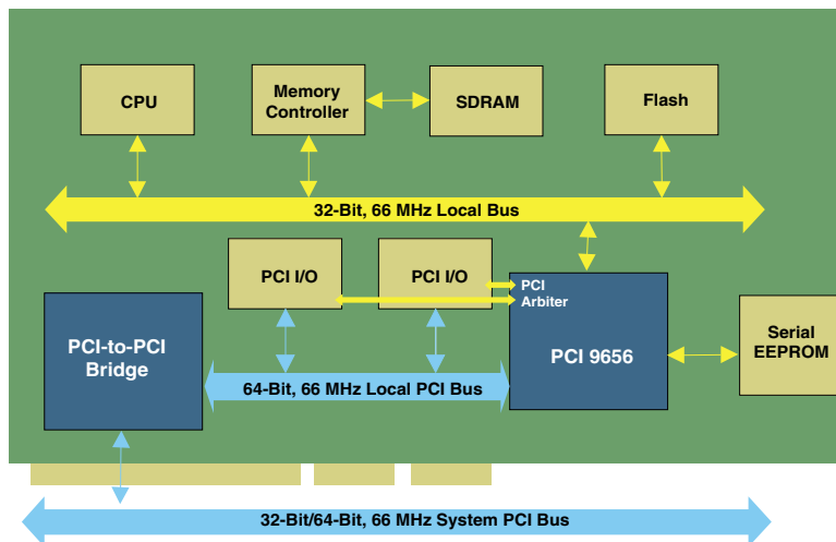
Figure 1-6. PCI 9656 PCI Adapter Card with Local PCI I/O and PCI-to-PCI Bridge
