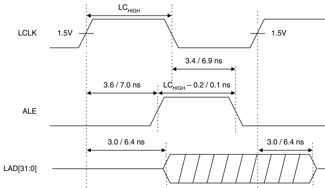
Figure 13-3. PCI 9656 ALE Output Delay to the Local Clock
