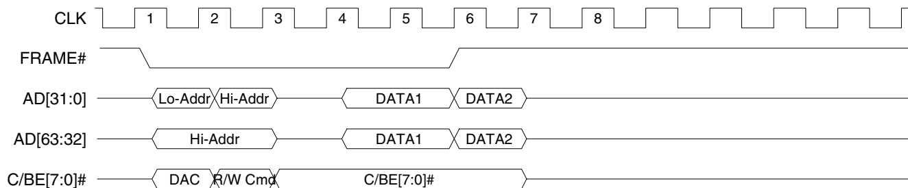
Figure 3-14. PCI Dual Address Cycle Timing
