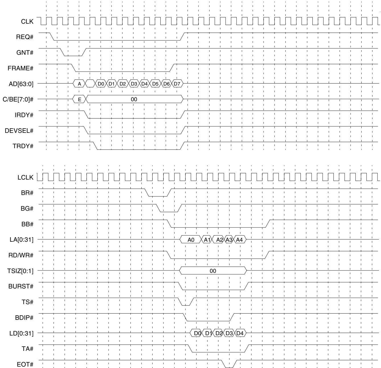
Timing Diagram 3-25. DMA PCI-to-Local, Continuous Burst Mode, with EOT# Assertion
