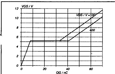
Fig. 14. Typical turn-on gate-charge characteristics. V_{GS} = f(Q_G) ; conditions: I_D = 11\text{ A} ; parameter V_{DS}
