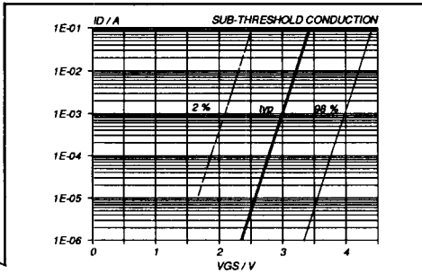
Fig. 12. Sub-threshold drain current. I_D = f(V_{GS}) ; conditions: T_j = 25^\circ\text{C} ; V_{DS} = V_{GS}
