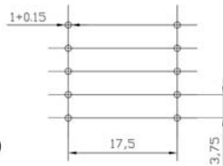
TOP VIEW Recommended PCB layout
