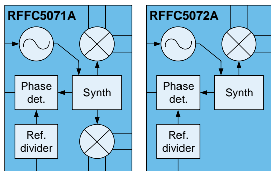
Functional Block Diagram – Simplified
