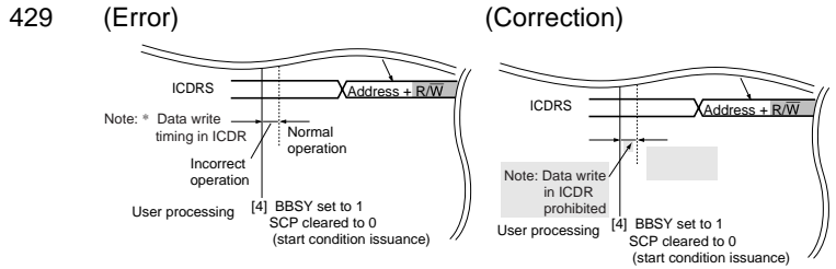
Figure 16.9 Example of Operation Timing in Master Transmit Mode (MLS = WAIT = 0)
