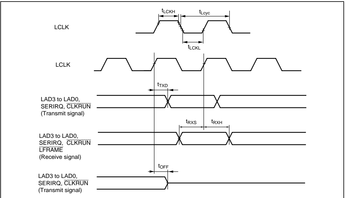
Figure 28.30 Host Interface (LPC) Timing
