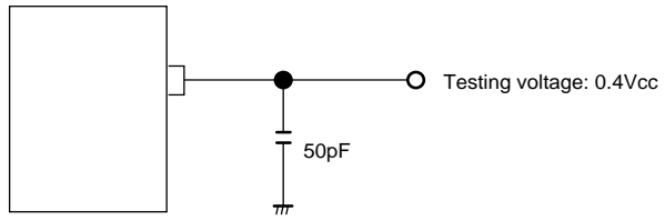
Figure 28.31 Tester Measurement Condition
