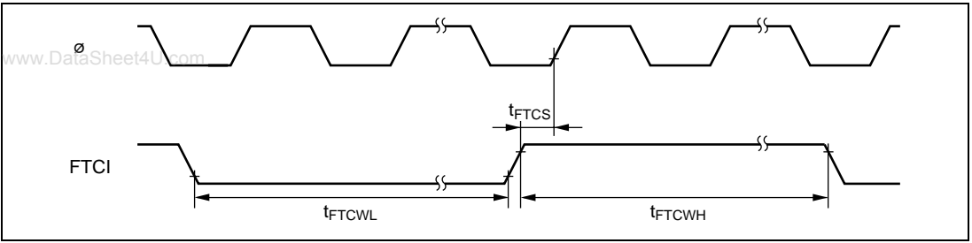
Figure 28.18 FRT Clock Input Timing
