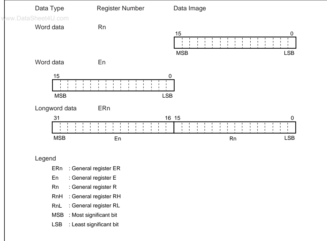
Figure 2.9 General Register Data Formats (2)
