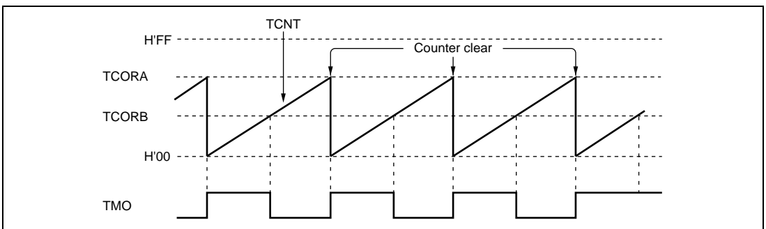
Figure 12.3 Pulse Output Example
