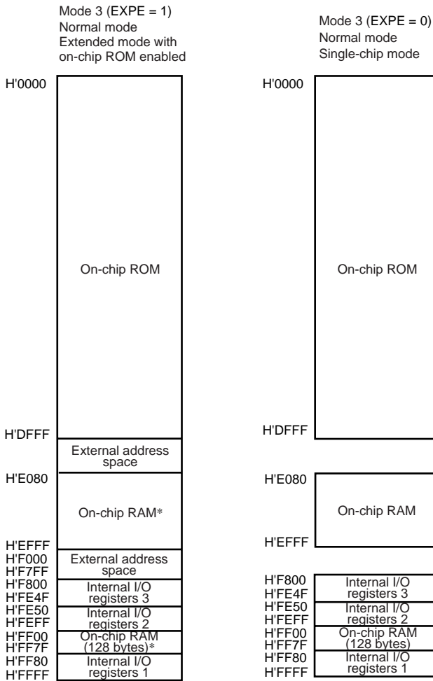
Figure 3.6 Address Map for H8S/2145BV (2)
