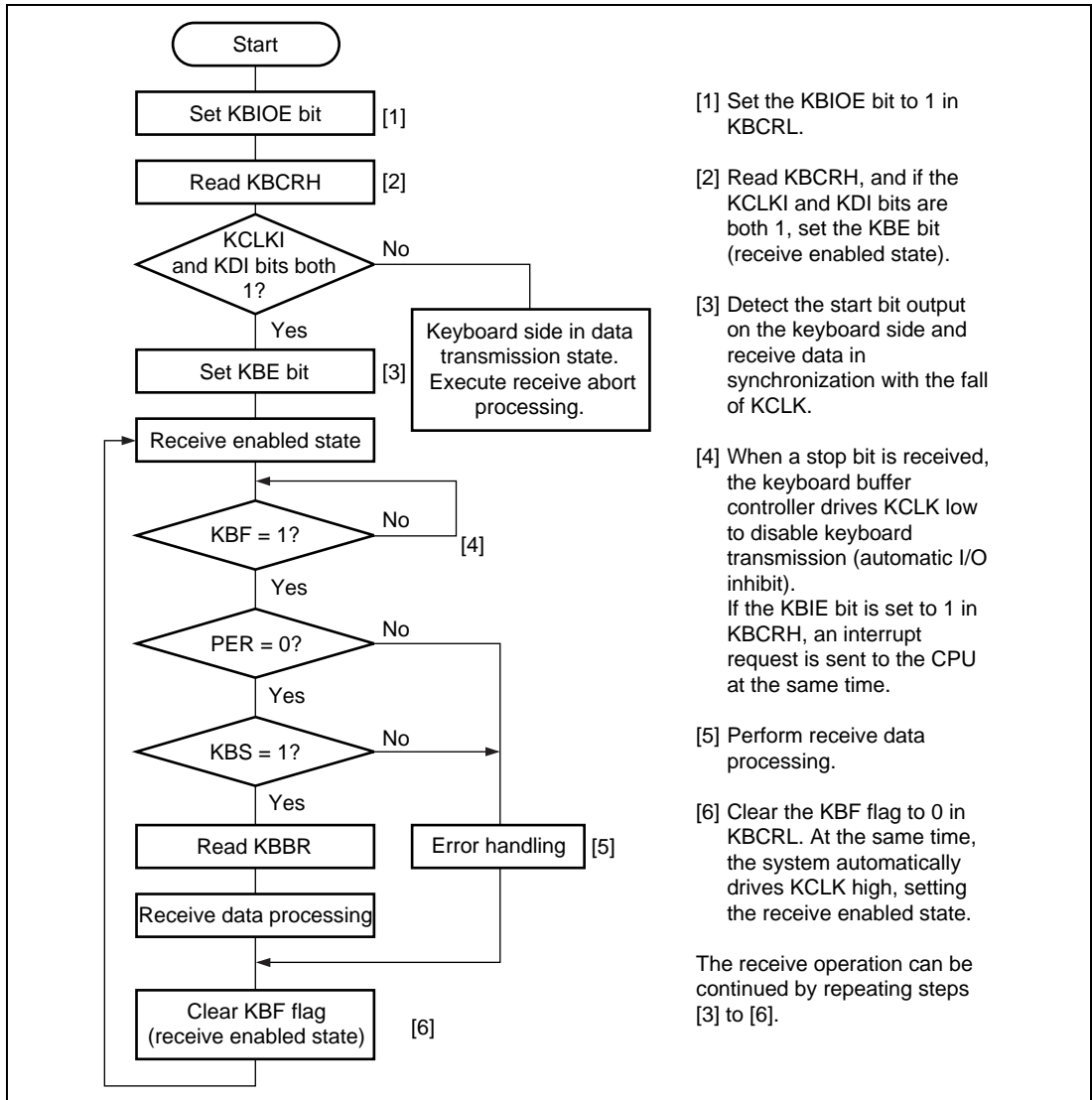
Figure 17.3 Sample Receive Processing Flowchart www.DataSheet4U.com
