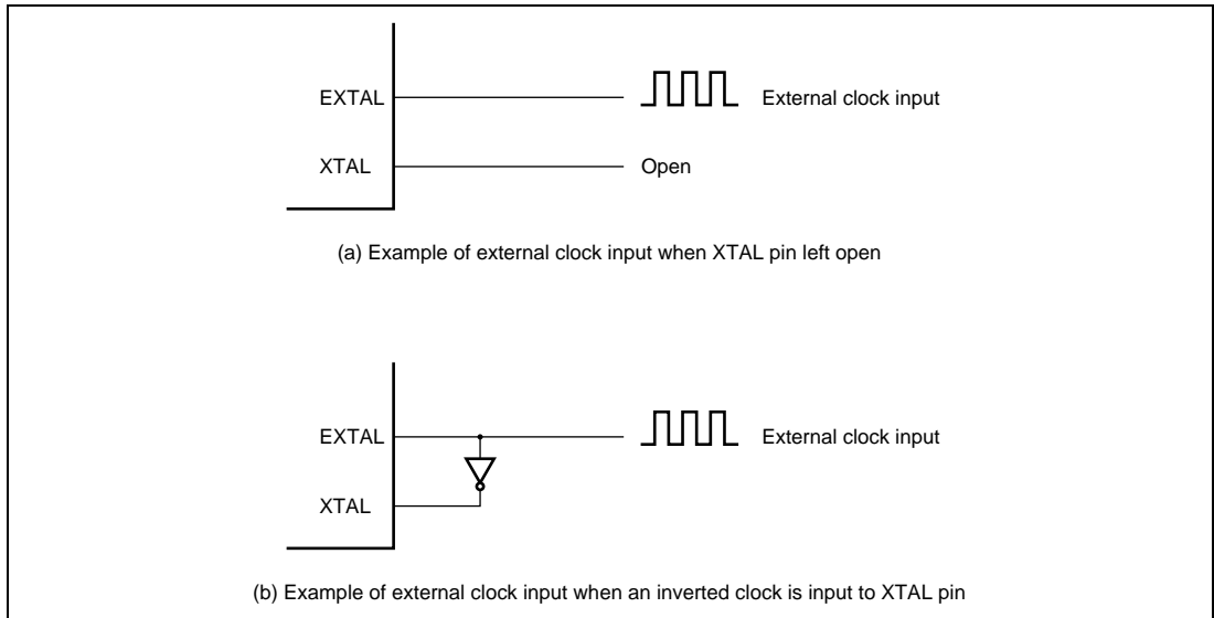
Figure 25.4 Example of External Clock Input
