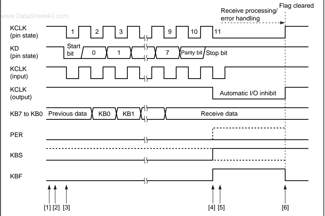
Figure 17.4 Receive Timing
