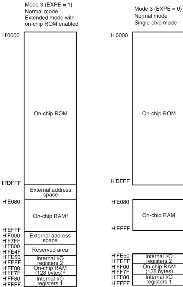
Figure 3.8 Address Map for H8S/2148B (2)
