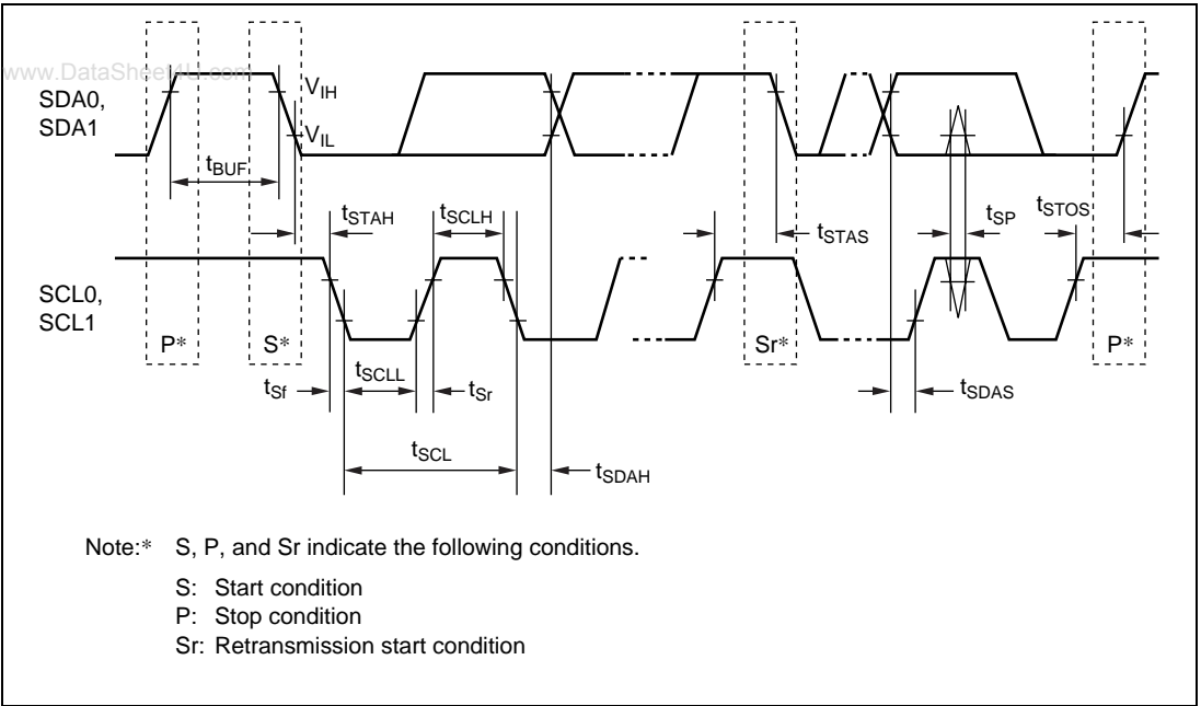
Figure 28.29 I 2 C Bus Interface Input/Output Timing
