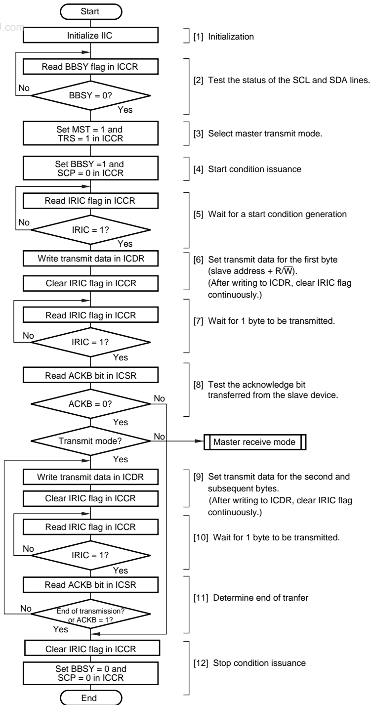
Figure 16.8 Sample Flowchart for Operations in Master
