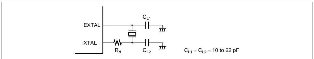
Figure 25.2 Typical Connection to Crystal Resonator
