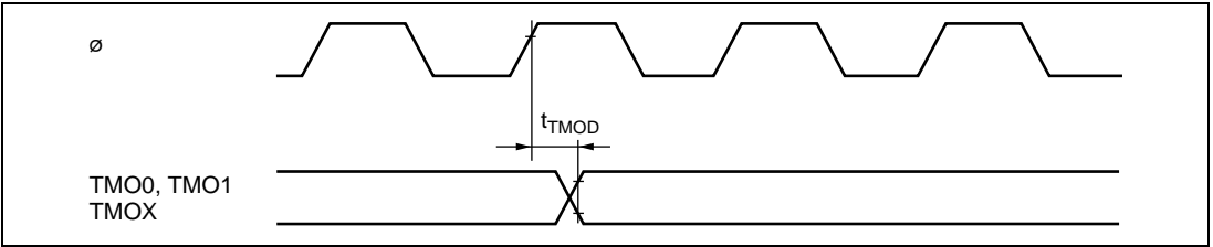
Figure 28.19 8-Bit Timer Output Timing
