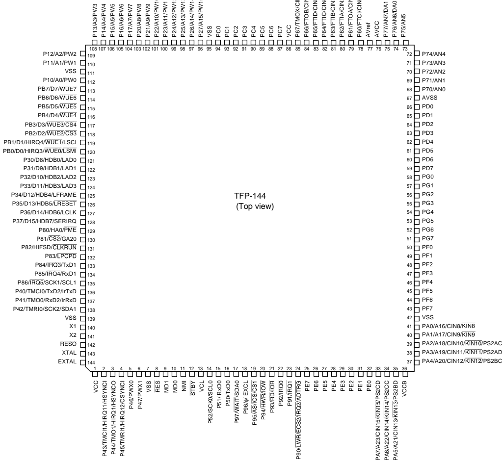
Figure 1.4 Pin Arrangement of H8S/2160B and H8S/2161B
