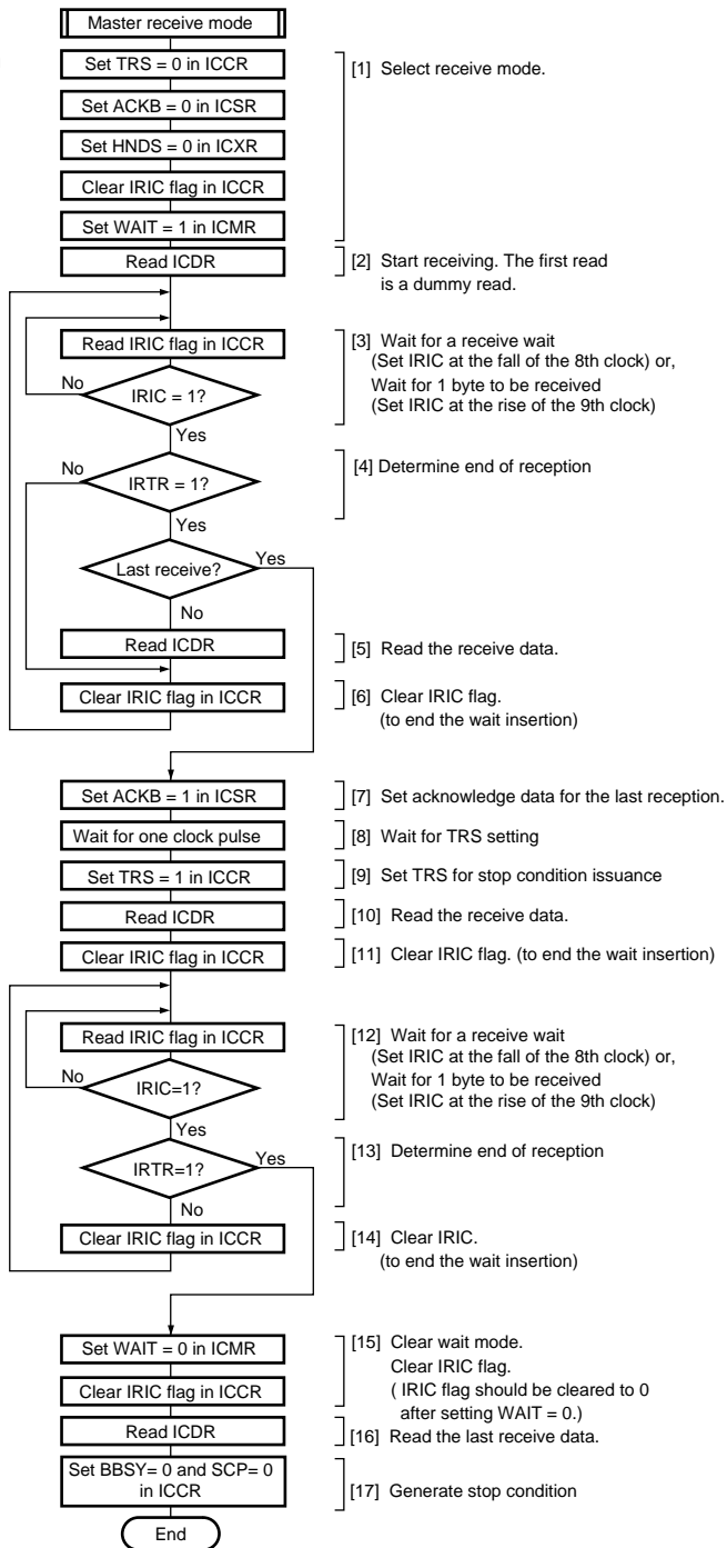
Figure 16.14 Sample Flowchart for Operations in Master Receive Mode (receiving multiple bytes) (WAIT = 1) www.DataSheet4U.com
