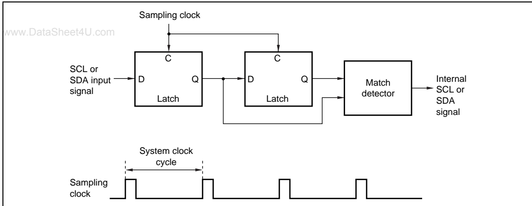
Figure 16.29 Block Diagram of Noise Canceler
