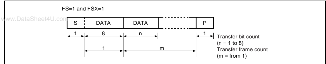
Figure 16.5 I 2 C Bus Data Format (Serial Format)
