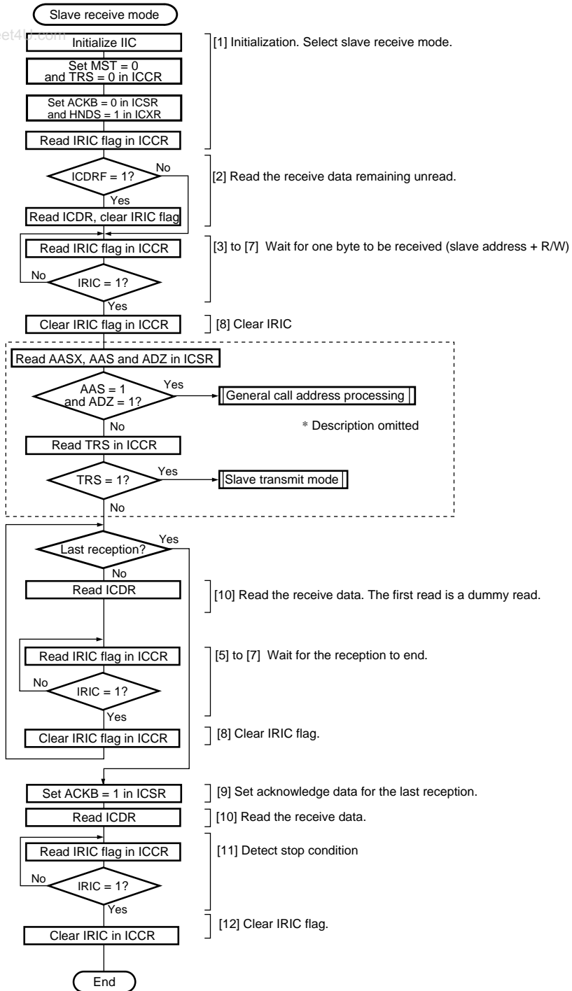
Figure 16.18 Sample Flowchart for Operations in Slave Receive Mode
