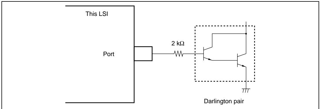
Figure 28.1 Darlington Pair Drive Circuit (Example)
