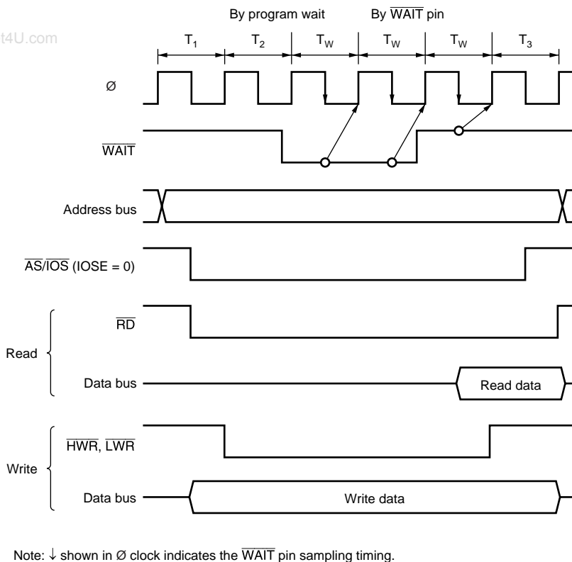
Figure 6.13 Example of Wait State Insertion Timing (Pin Wait Mode)
