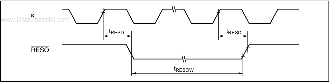
Figure 28.26 WDT Output Timing ( \overline{\text{RESO}} )
