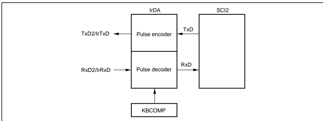
Figure 15.21 IrDA Block Diagram
