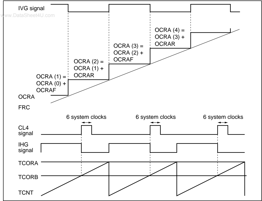
Figure 13.8 IVG Signal/IHG Signal/CL4 Signal Timing Chart
