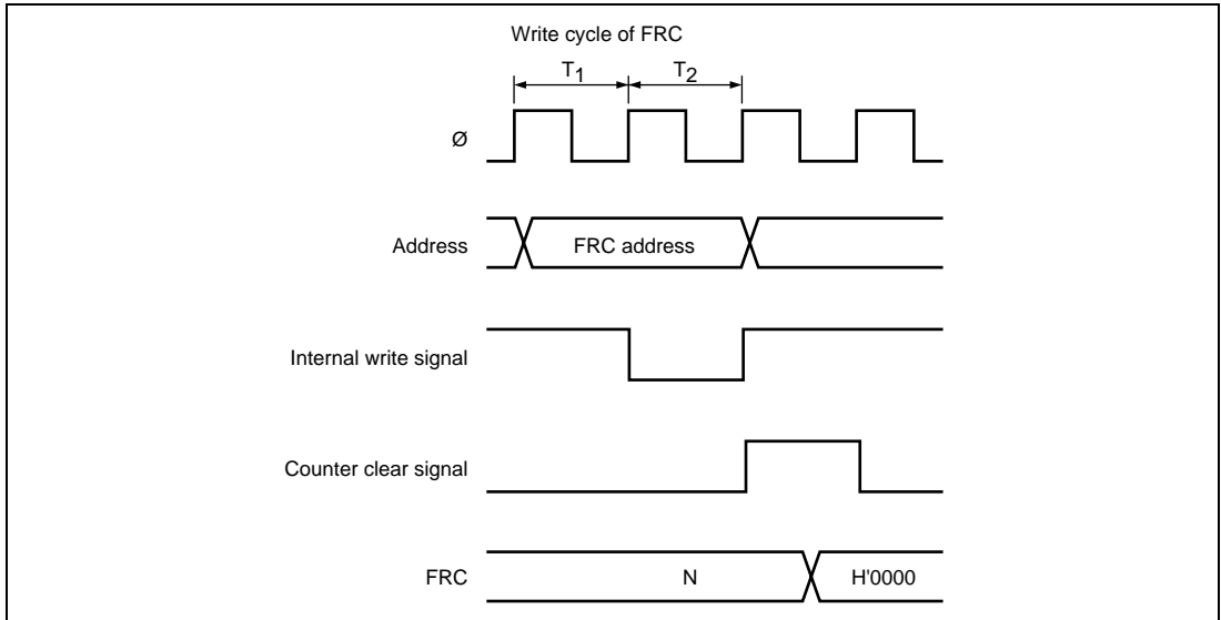
Figure 11.17 FRC Write-Clear Conflict
