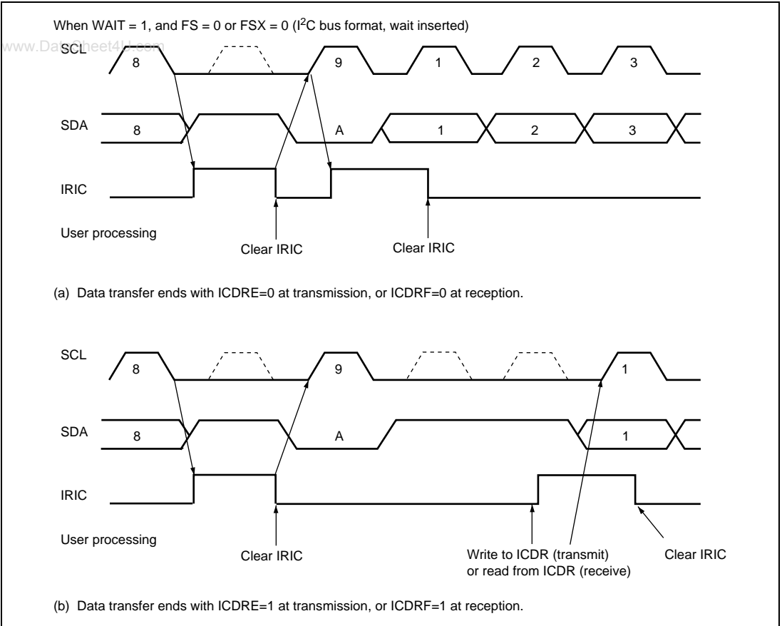
Figure 16.27 IRIC Setting Timing and SCL Control (2)
