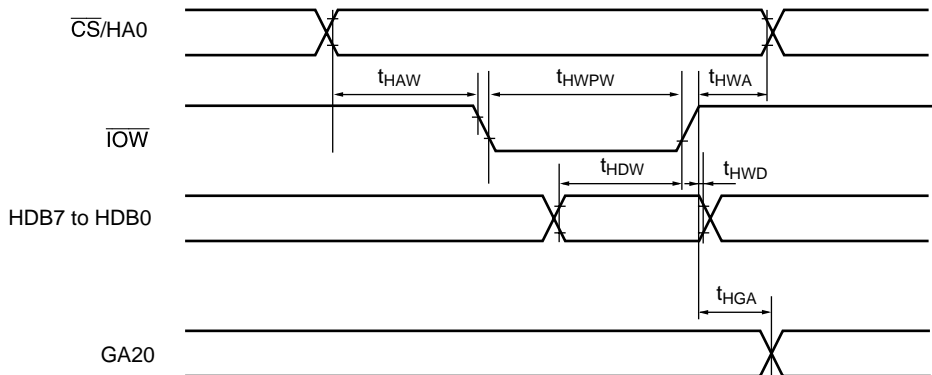
Figure 28.27 Host Interface (XBS) Timing
