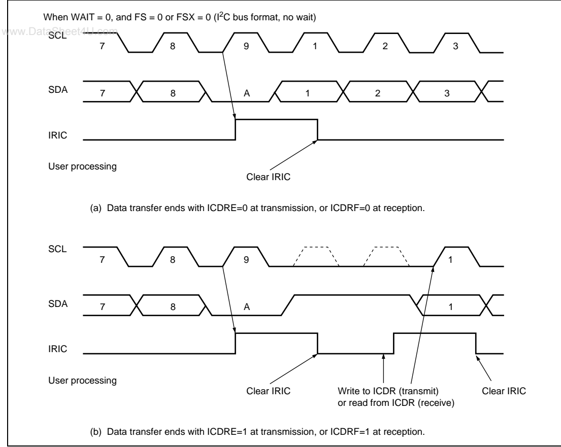
Figure 16.26 IRIC Setting Timing and SCL Control (1)
