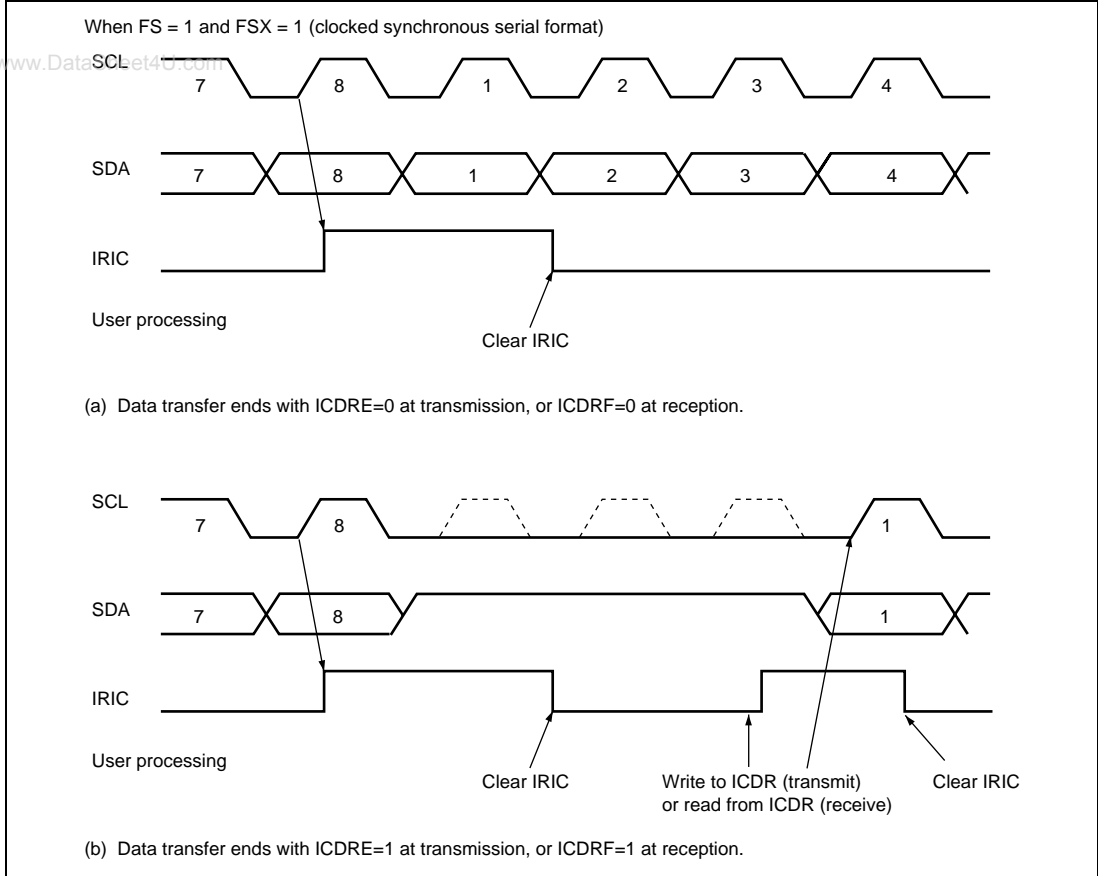
Figure 16.28 IRIC Setting Timing and SCL Control (3)
