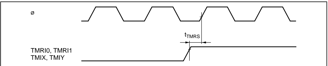
Figure 28.21 8-Bit Timer Reset Input Timing
