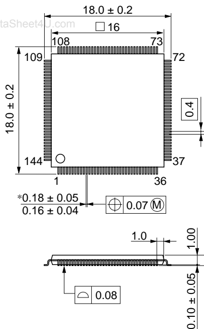
Figure C.3 Package Dimensions (TFP-144)
