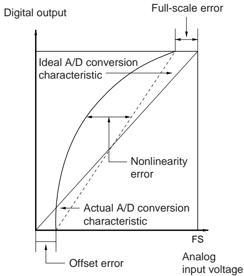
Figure 21.6 A/D Conversion Accuracy Definitions
