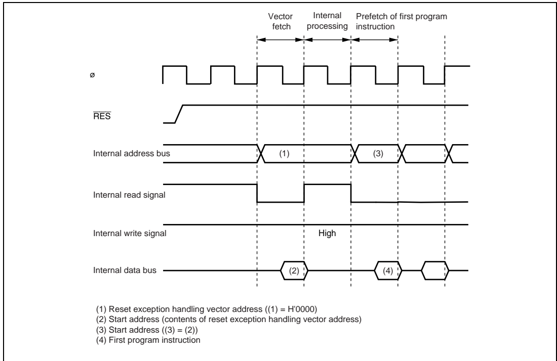
Figure 4.1 Reset Sequence (Mode 3) www.DataSheet4U.com
