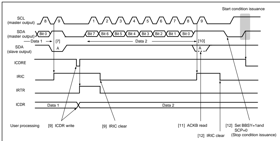
Figure 16.10 Example of Stop Condition Issuance Operation Timing
