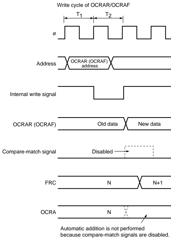
Figure 11.20 Conflict between OCRAR/OCRAF Write and Compare-Match (When Automatic Addition Function is Used)
