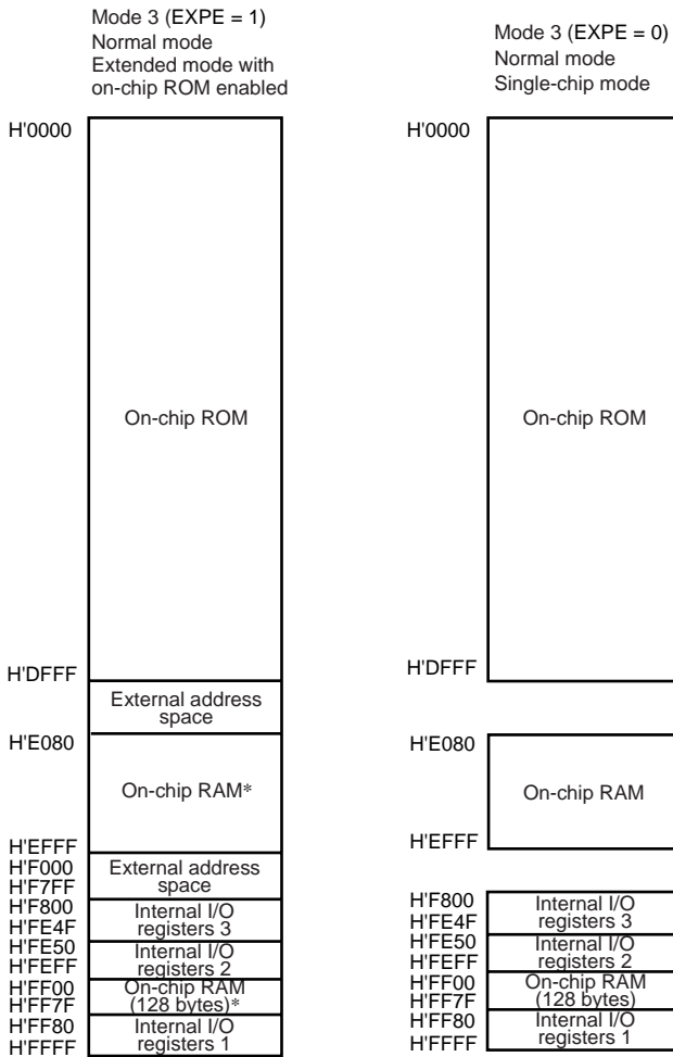
Figure 3.4 Address Map for H8S/2141B and H8S/2161B (2)
