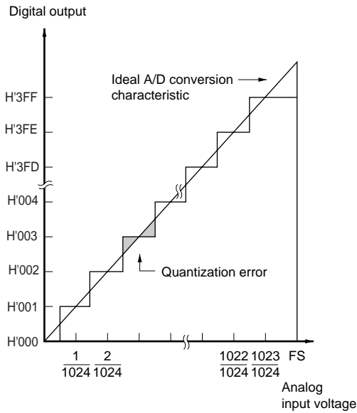
Figure 21.5 A/D Conversion Accuracy Definitions
