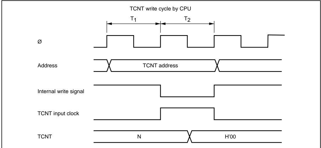
Figure 12.14 Conflict between TCNT Write and Clear
