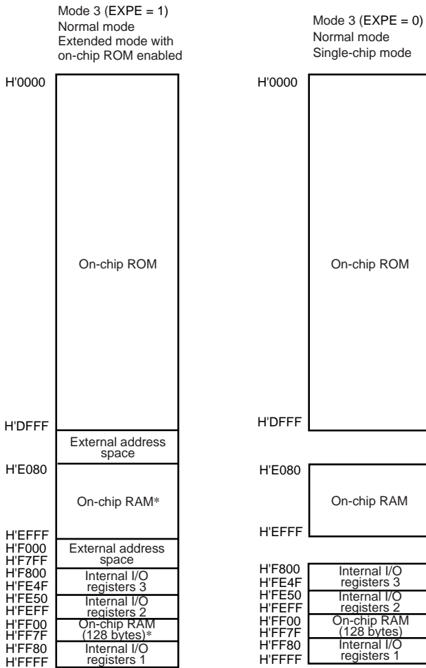
Figure 3.2 Address Map for H8S/2140B and H8S/2160B (2)
