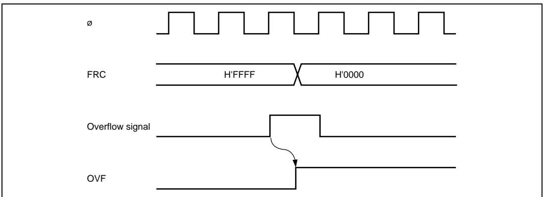
Figure 11.13 Timing of Overflow Flag (OVF) Setting
