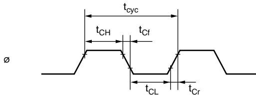
Figure 28.6 System Clock Timing
