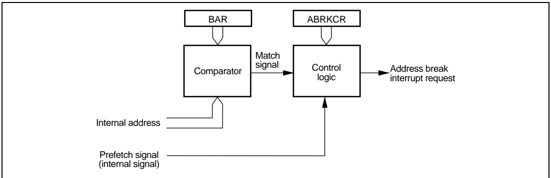
Figure 5.9 Address Break Block Diagram
