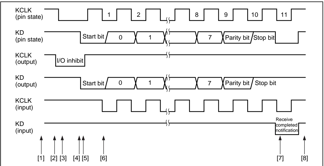
Figure 17.6 Transmit Timing
