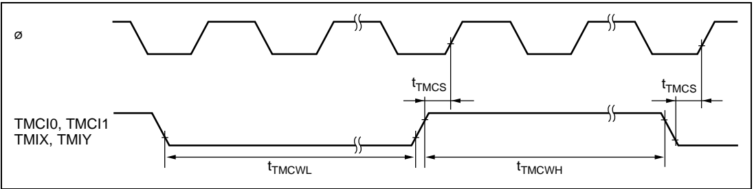
Figure 28.20 8-Bit Timer Clock Input Timing
