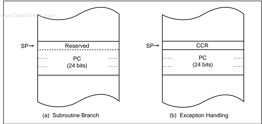
Figure 2.4 Stack Structure in Advanced Mode
