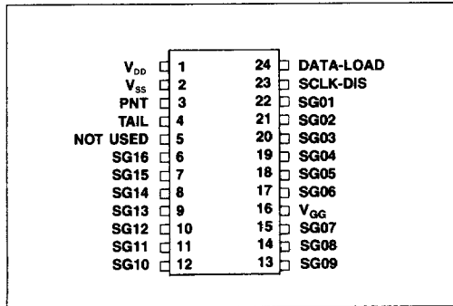
10941 Pin Configuration
