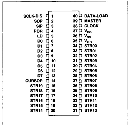
10939 Pin Configuration
