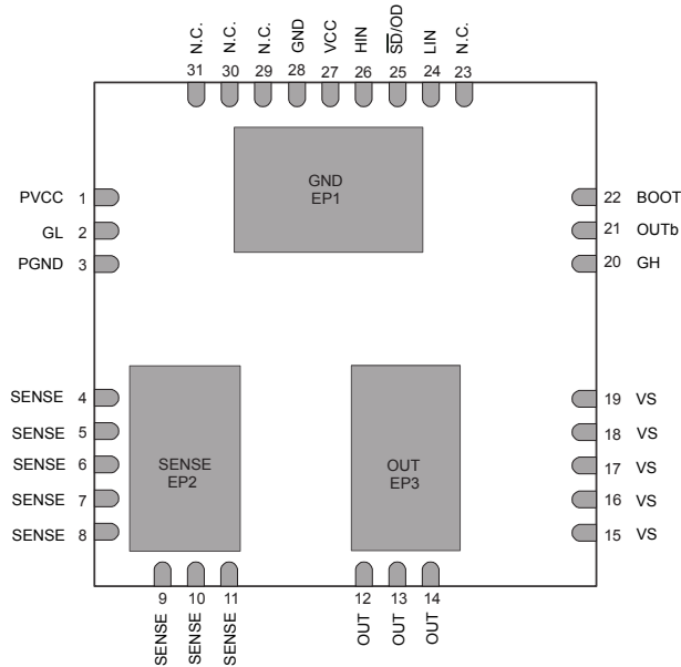
Figure 2. Pin connections (top view)
