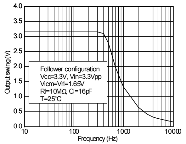
Figure 13. Output swing vs. input signal frequency
