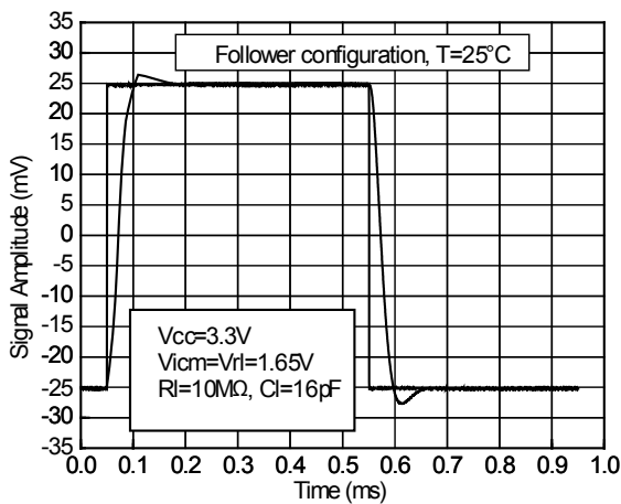
Figure 14. Small signal response at 3.3 V supply voltage
