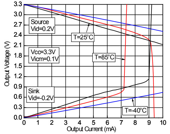
Figure 9. Output characteristics at 3.3 V supply voltage
