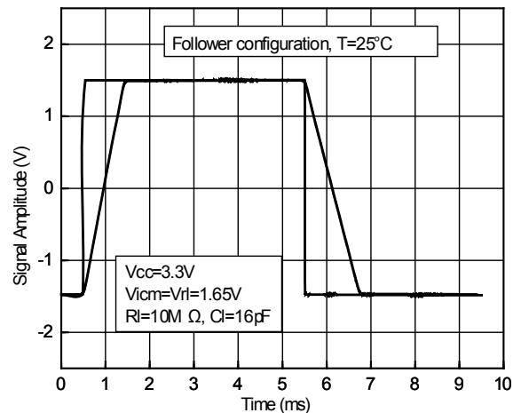
Figure 15. Large signal response at 3.3 V supply voltage
