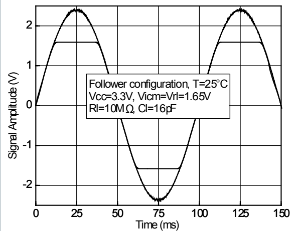
Figure 11. Phase reversal free
