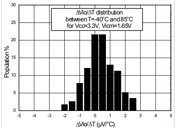
Figure 7. Input offset voltage temperature coefficient distribution
