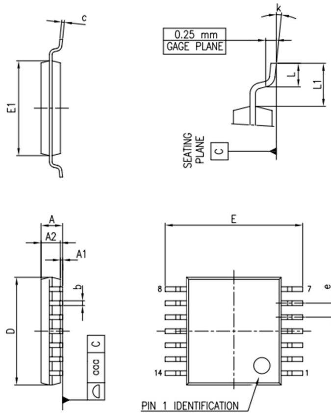
Figure 22. TSSOP-14 package outline
