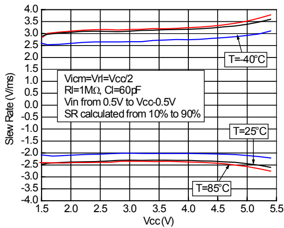
Figure 12. Slew rate vs. supply voltage
