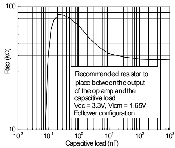
Figure 18. R_{iso} to drive capacitors above 100 pF in follower configuration
