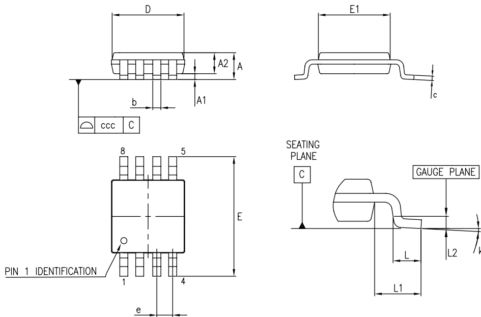
Figure 21. MiniSO8 package outline
