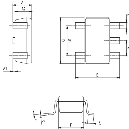
Figure 20. SOT23-5 package outline
