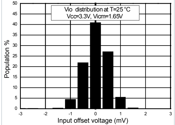
Figure 5. Input offset voltage distribution
