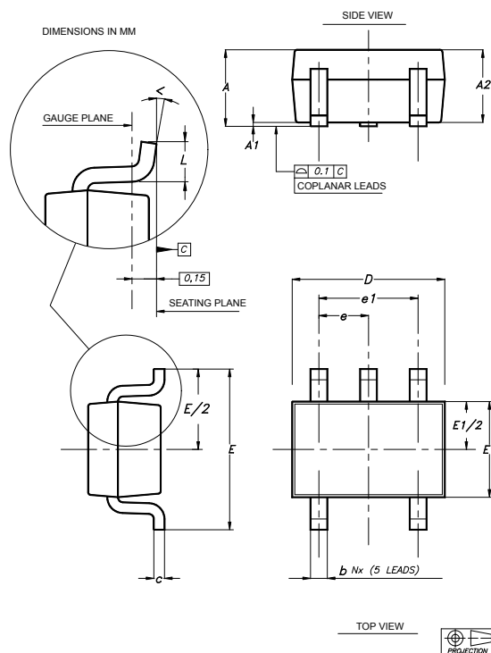
Figure 19. SC70-5 (or SOT323-5) package outline
