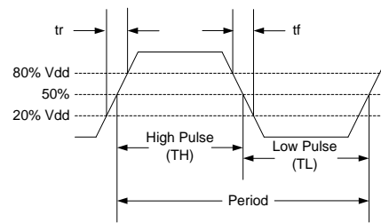
Figure 3. Waveform [8]
