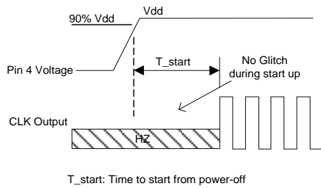
Figure 4. Startup Timing [9]
