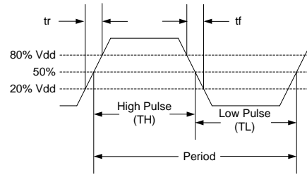
Figure 3. Waveform [10]
