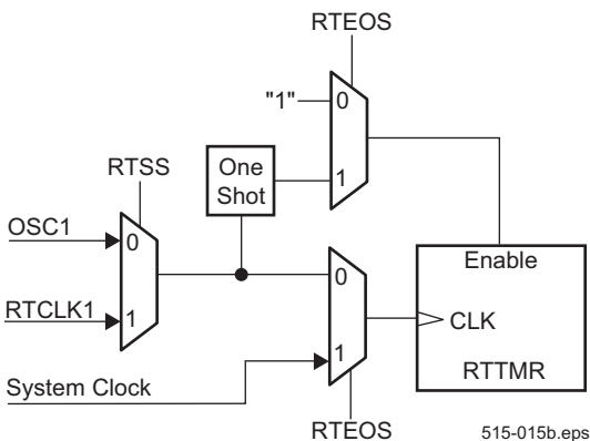
Figure 5-4 Real-Time Timer Block Diagram
